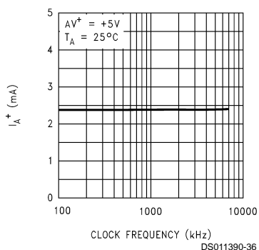
Analog Supply Current ( I_A ) vs Clock Frequency
