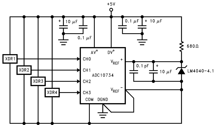
FIGURE 15. Different Reference Configurations
