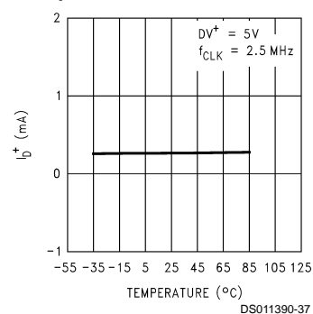
Digital Supply Current ( I_D ) vs Temperature
