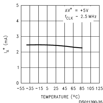
Analog Supply Current ( I_A ) vs Temperature
