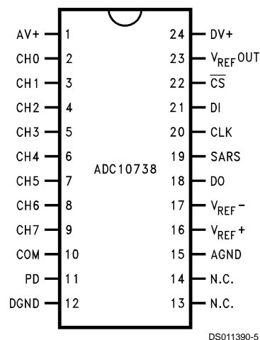
Top View See NS Package Number M24B
