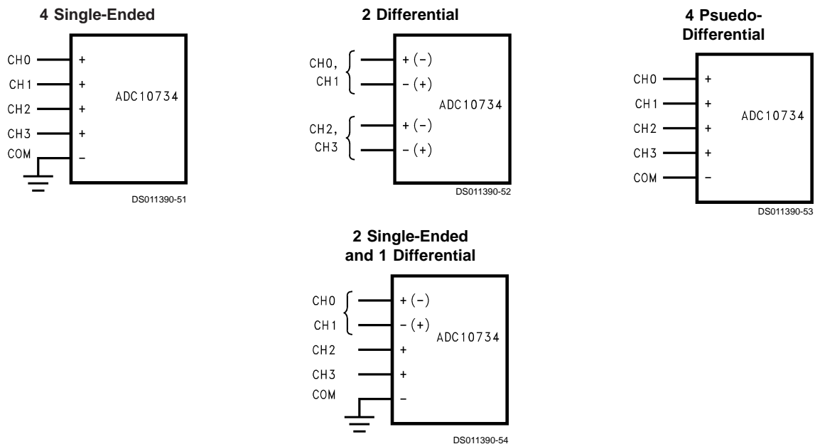
FIGURE 13. Analog Input Multiplexer Options
