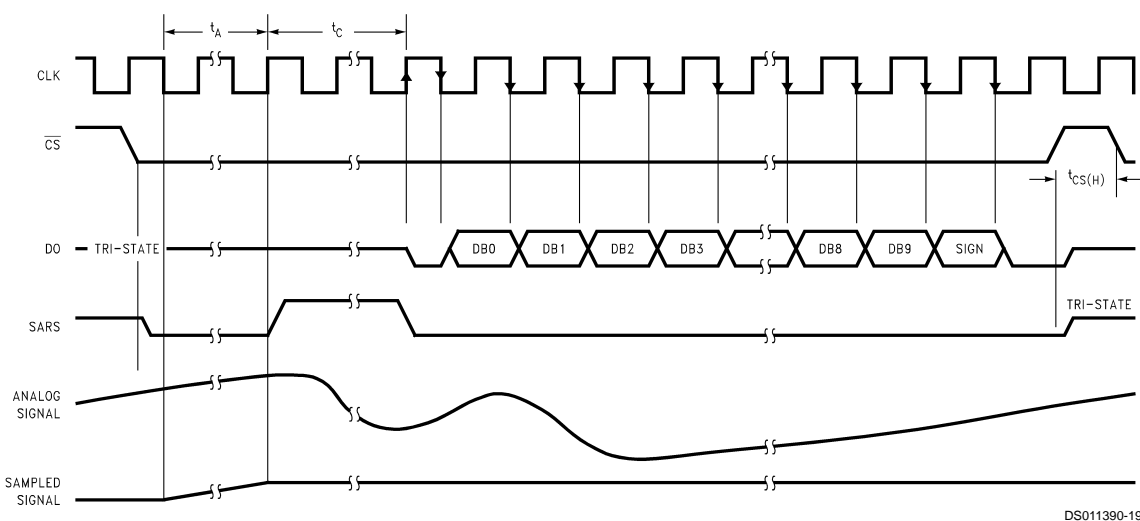
FIGURE 8. ADC10731 \overline{CS} Low during Conversion
