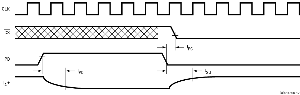
FIGURE 6. Hardware Power Up/Down Sequence
