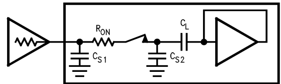
FIGURE 16. Analog Input Model
