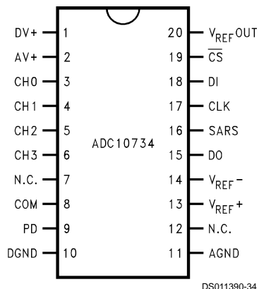
See NS Package Number MSA20
