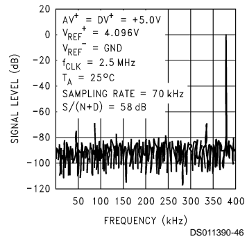
Power Bandwidth Response with 380 kHz Sine Wave
