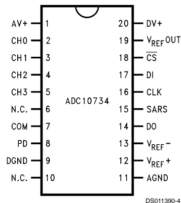
Top View See NS Package Number M20B
