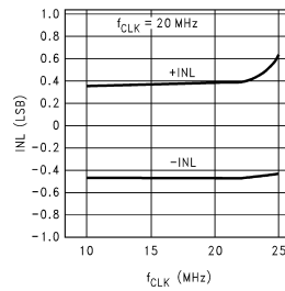
INL vs f_{\text{CLK}}
