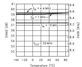
SINAD & ENOB vs Temperature and f_{\text{IN}}
