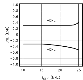
DNL vs f_{\text{CLK}}
