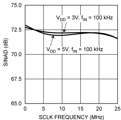
ADC121S101 SINAD vs. f_{SCLK}
