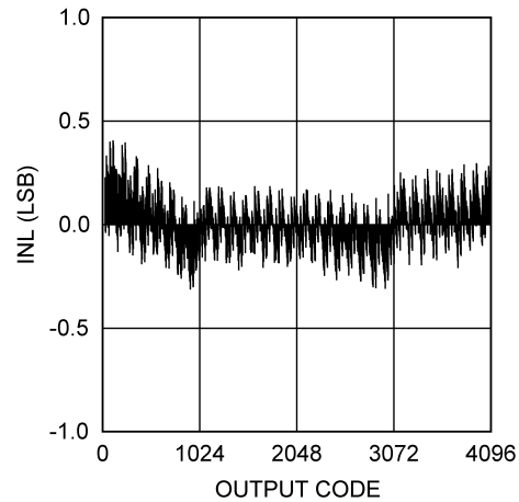
ADC121S101 INL
