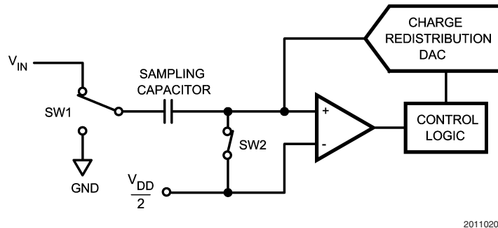
FIGURE 5. ADC121S101/101S101/081S101 in Track Mode
