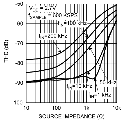
ADC121S101 THD vs. Source Impedance
