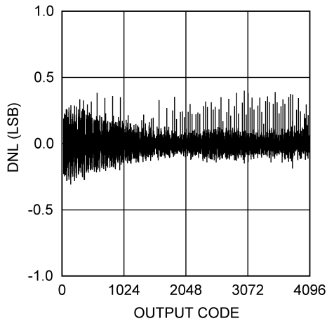
ADC121S101 DNL
