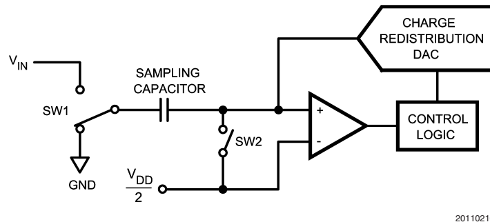
FIGURE 6. ADC121S101/101S101/081S101 in Hold Mode
