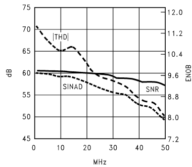
Dynamics at 27 MSPS
