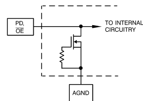
CLOCK PIN PROTECTION
