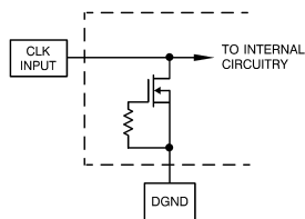
CLOCK PIN PROTECTION
