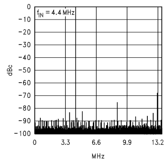
Spectral Response at 27 MSPS
