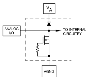
ANALOG PIN PROTECTION
