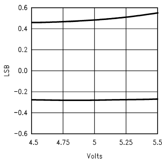
DNL vs V_A
