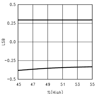
DNL vs Clock Duty Cycle
