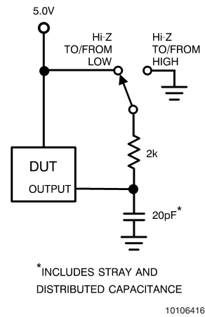
FIGURE 3. t_{EN} , t_{DIS} Test Circuit
