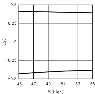
INL vs Clock Duty Cycle
