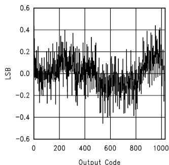
Typical INL
