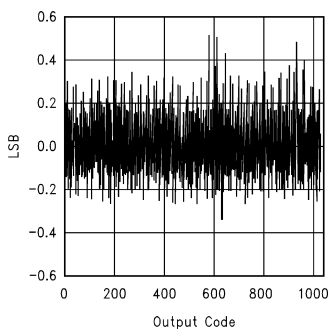
Typical DNL
