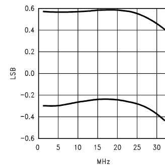
DNL vs f_{CLK}
