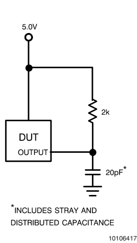
FIGURE 2. AC Test Circuit
