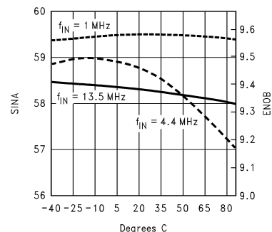
SINAD & ENOB vs Temperature and f_{IN}
