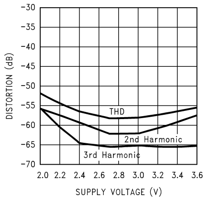
Distortion vs. Supply Voltage, V_A
