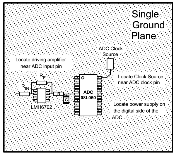
FIGURE 5. Layout Example
