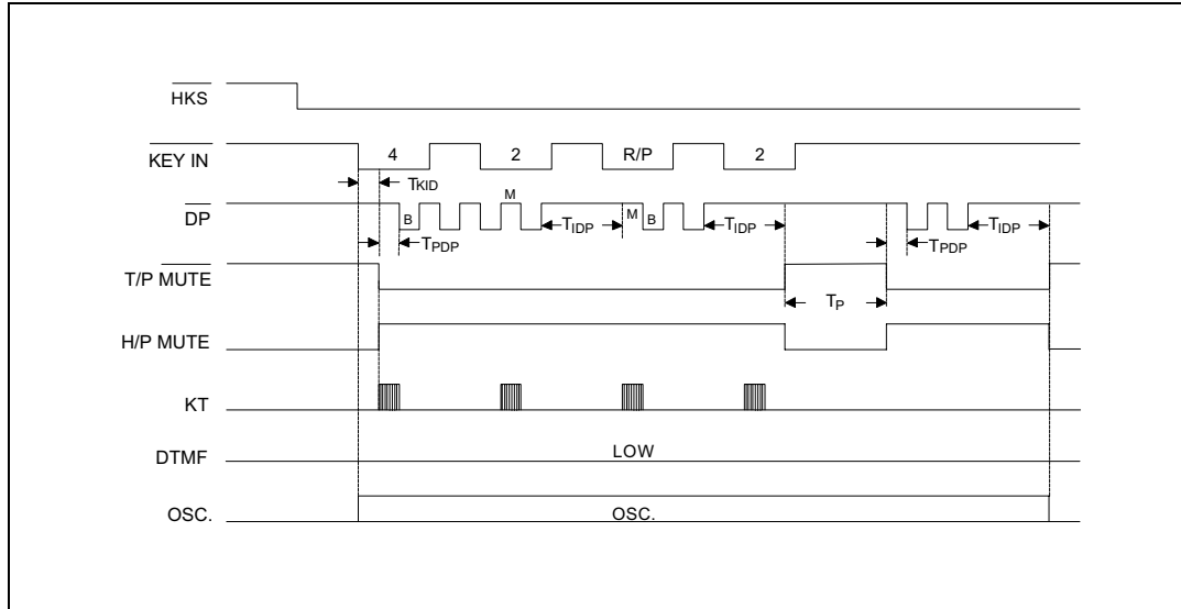
Figure 6 Pause Function Timing Diagram
