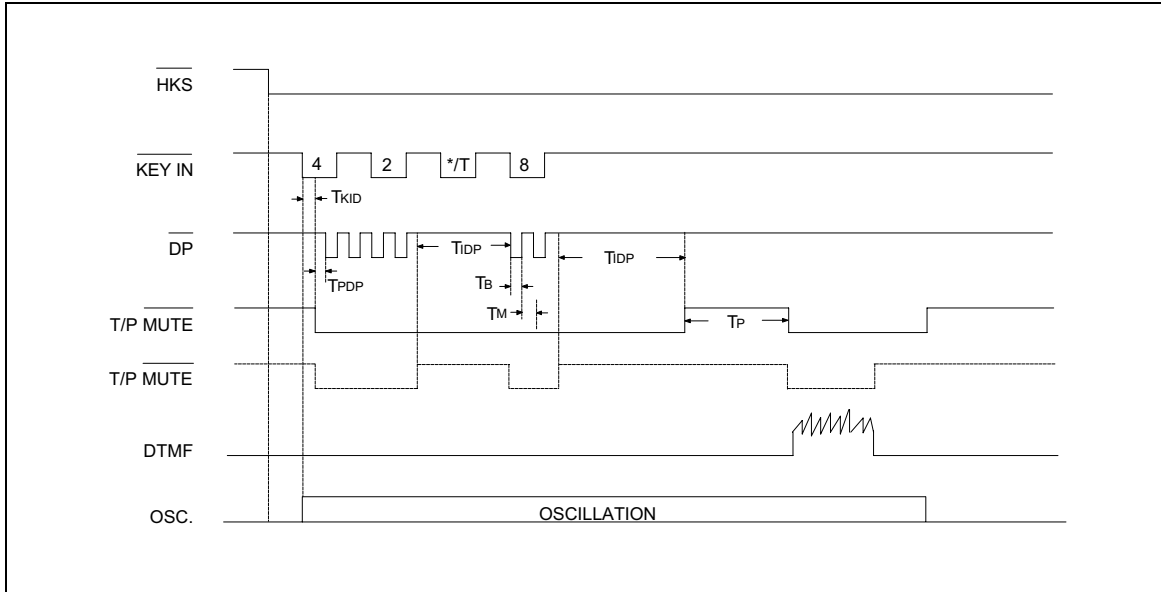
Figure 4(a). P→T Operation Timing Diagram in Normal Dialing (W91212, W91216)
