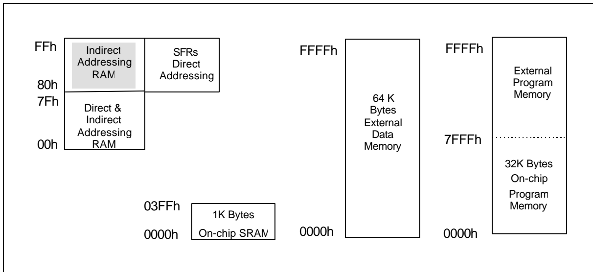
Figure 1. Memory Map
