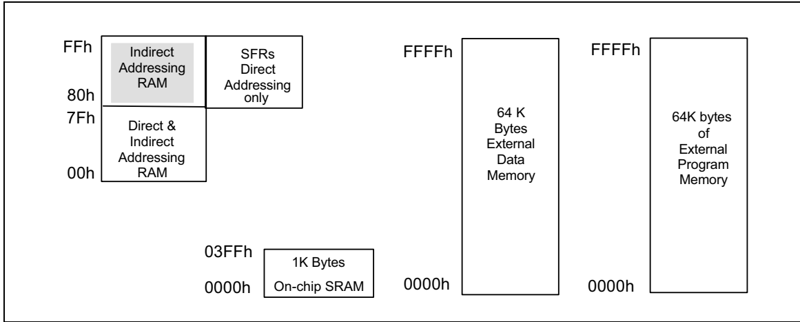
Figure 1. Memory Map
