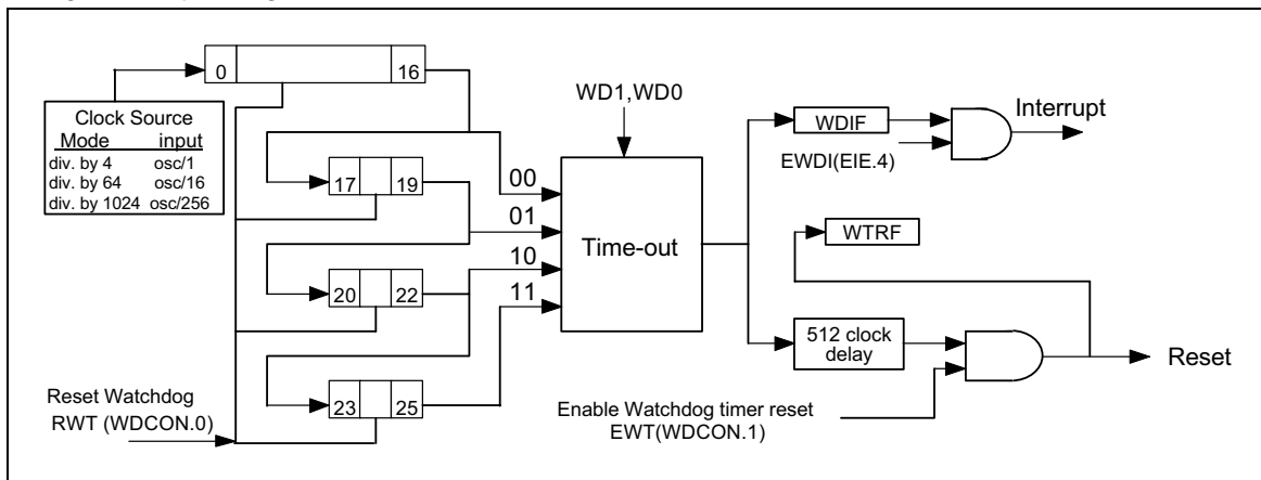
Figure 19. Watchdog Timer
