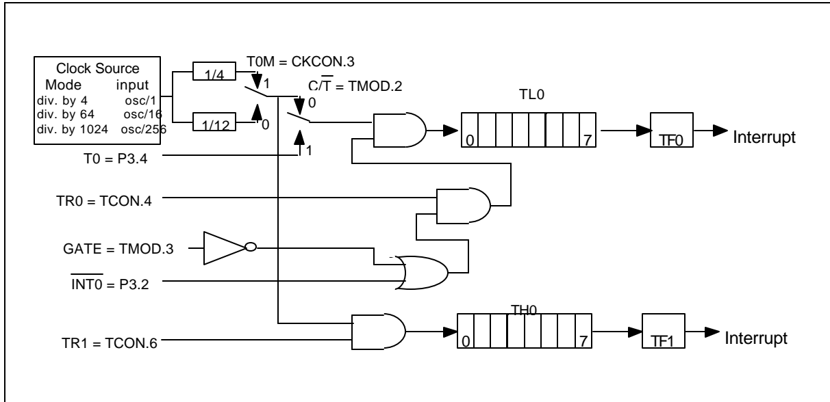
Figure 13. Timer/Counter 0 Mode 3
