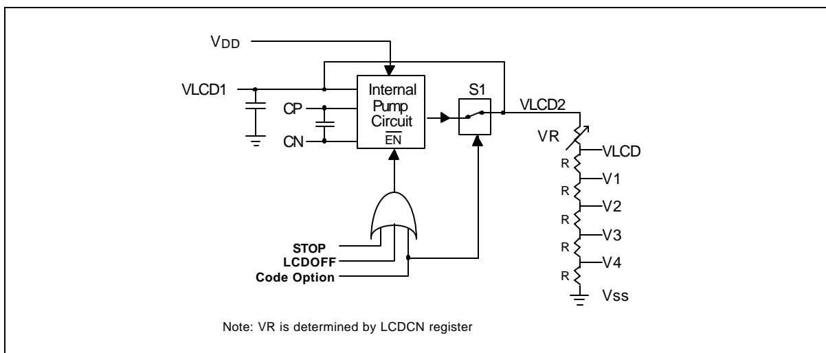
Figure 5-18 LCD power control circuit
