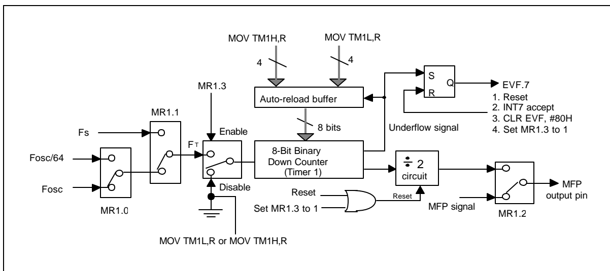
Figure 5-7 Organization of Timer 1
