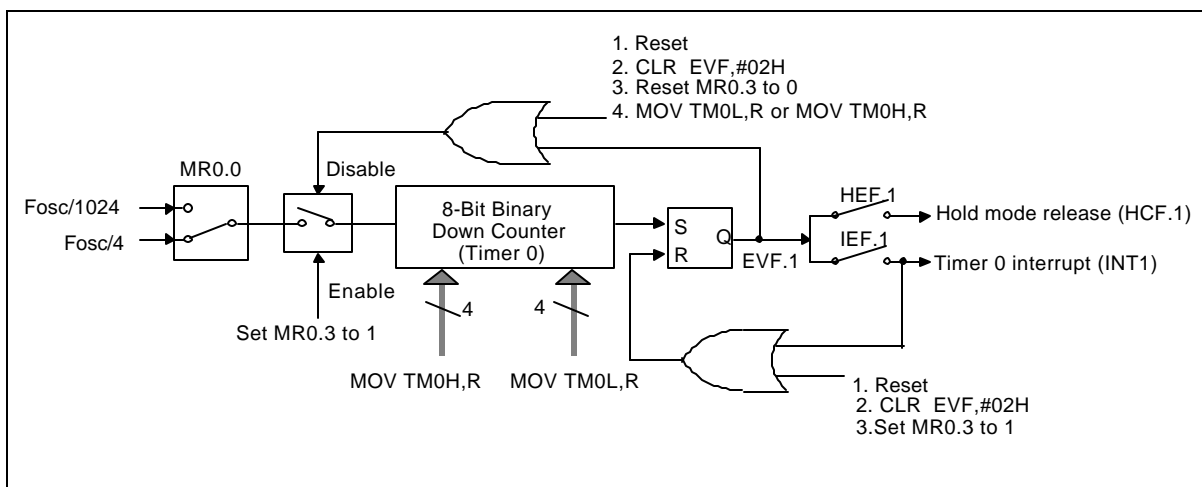
Figure 5-6 Organization of Timer 0
