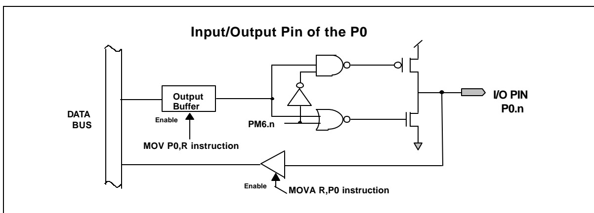
Figure 5-11 Architecture of P0 Input/Output pins
