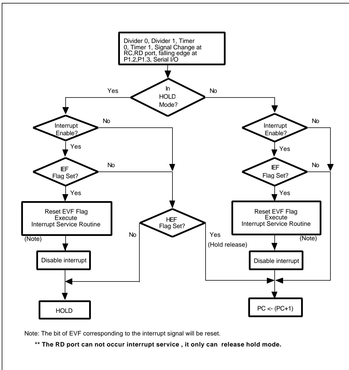
Figure 5-9 Hold Mode and Interrupt Operation Flow Chart
