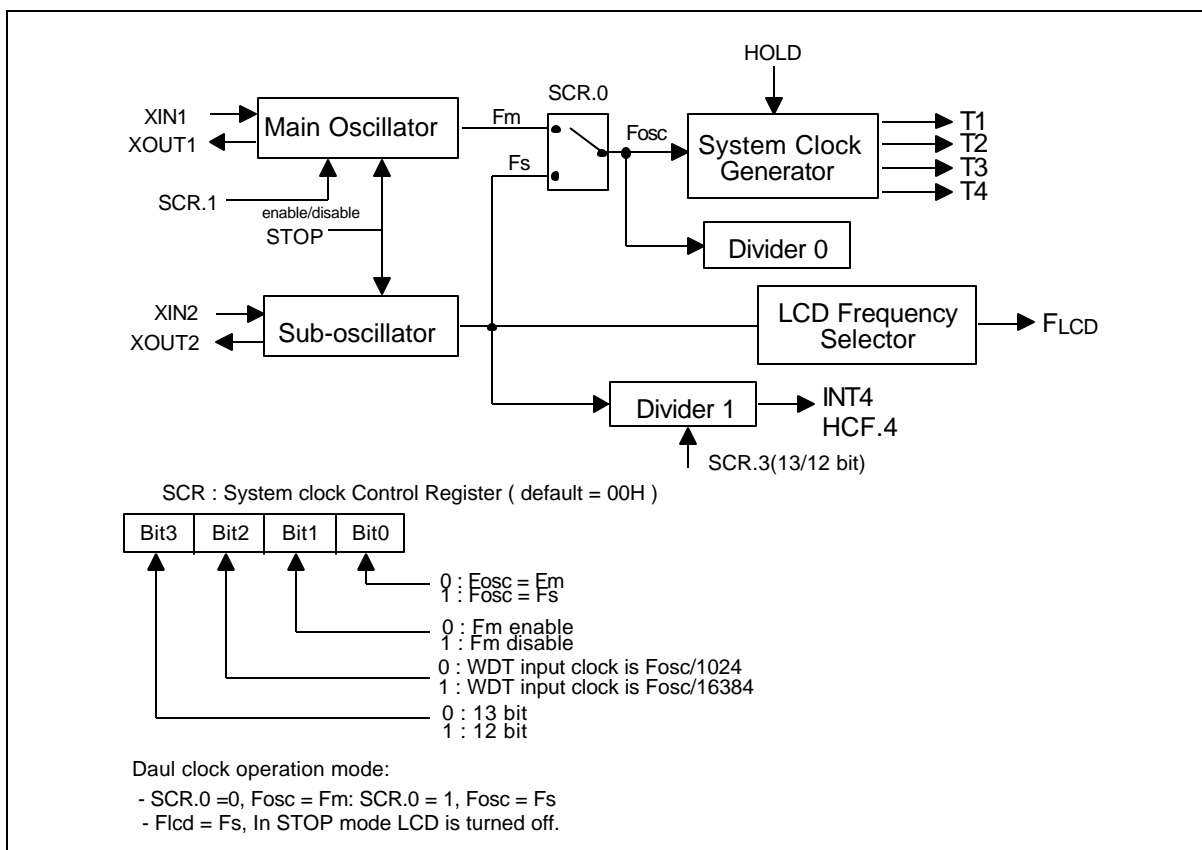
Figure 5-4 Organization of the dual-clock operation mode
