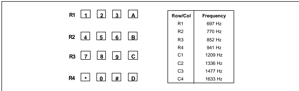
Figure 5-16 The relation between the touch tone keypad and the frequency
