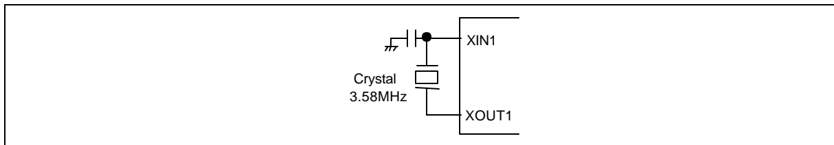
Figure 5-3 System clock oscillator Configuration
