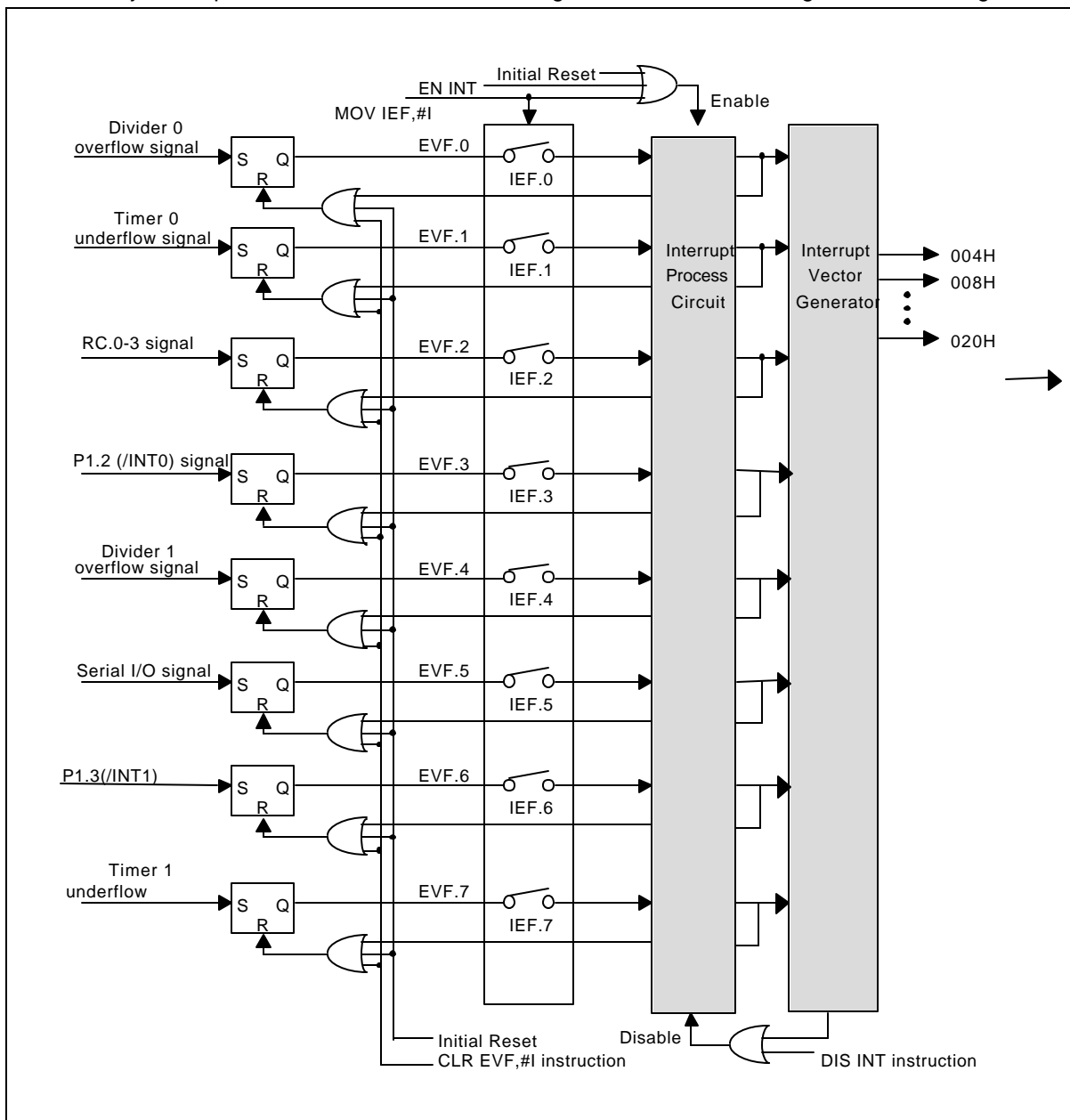
Figure 5-8 Interrupt event control diagram
