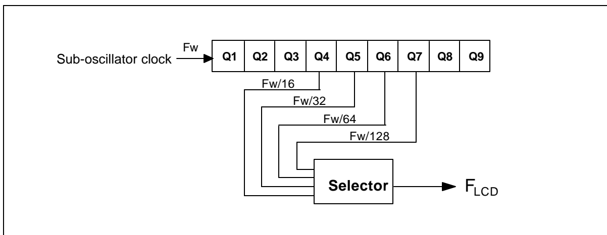
Figure 5-17 LCD alternating frequency (FLCD) circuit diagram
