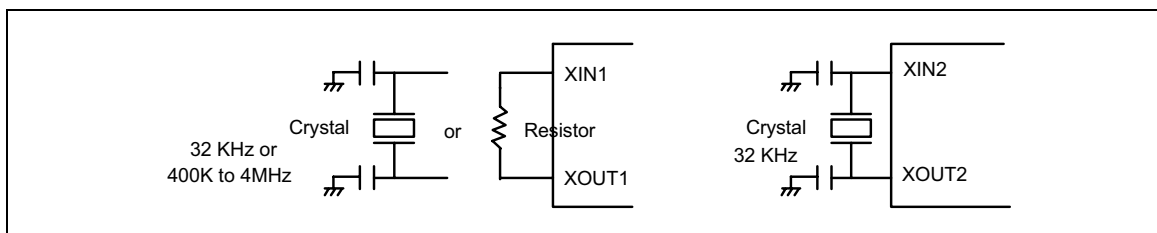
Figure 3. Oscillator Configuration
