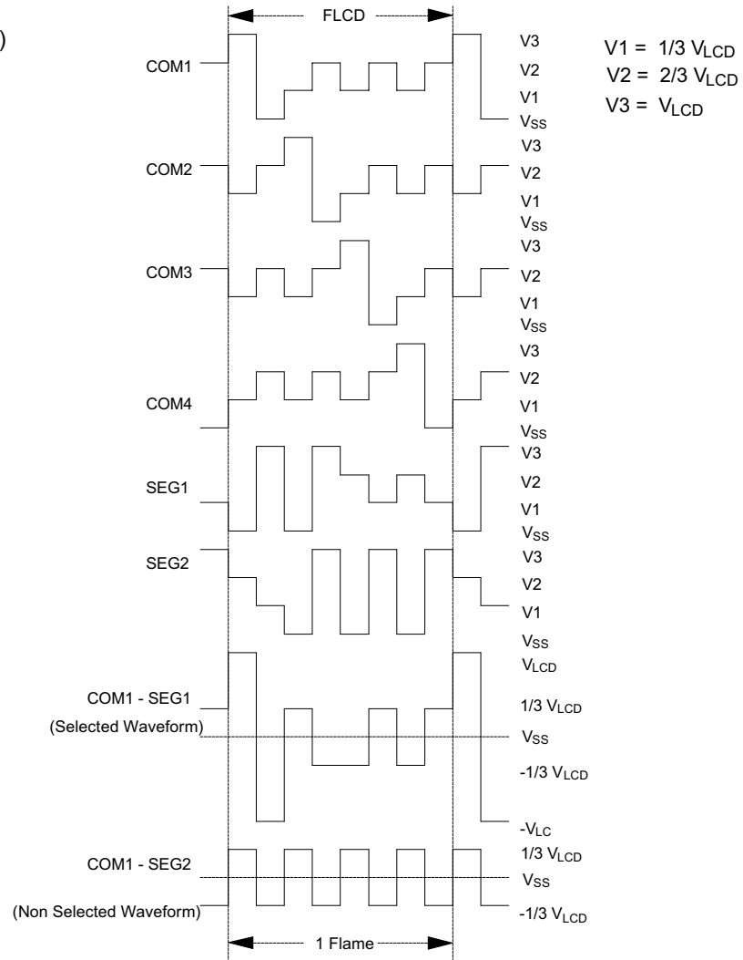
Figure 10. LCD Waveform
