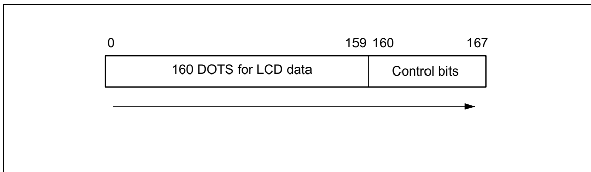
Figure 1. Address Format
