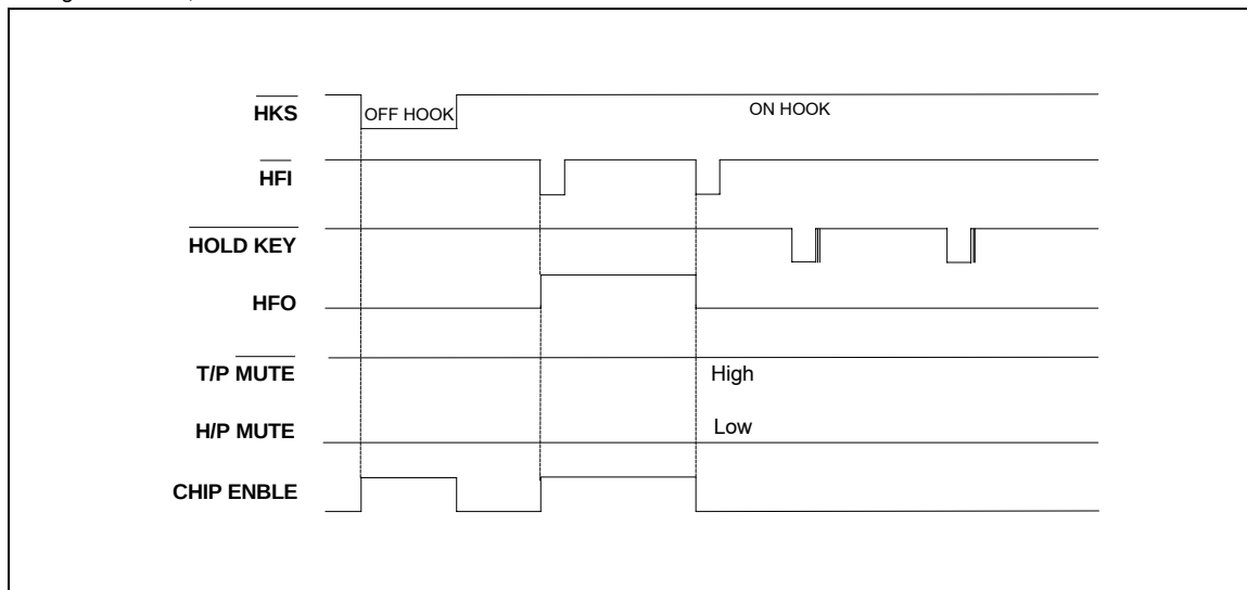
Figure 8(a). Hold and Handfree Timing Diagram
