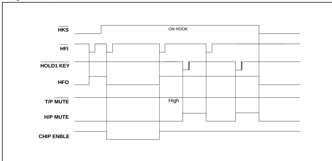
Figure 8(c). Hold and Handfree Timing Diagram
