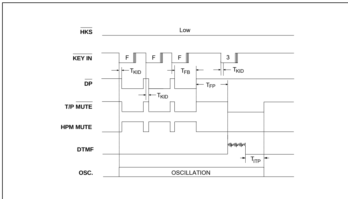
Figure 7. First Priority Flash Timing Diagram
