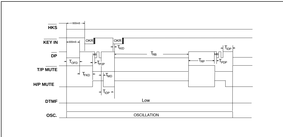
Figure 3. One-key Redial Timing Diagram
