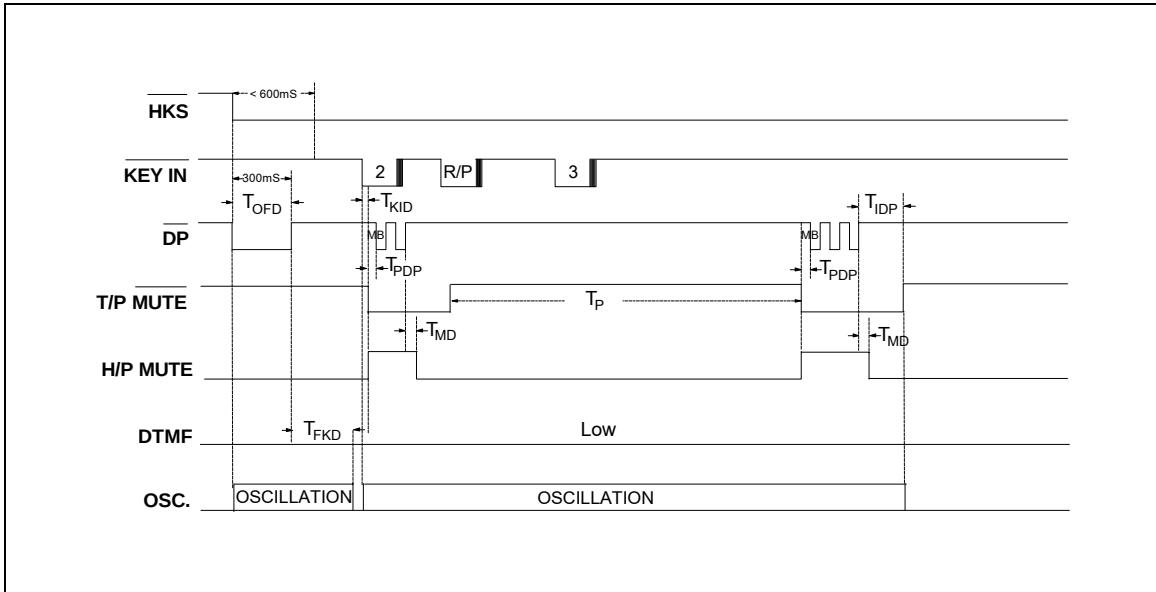
Figure 5. Pause Function Timing Diagram (Pulse Mode)
