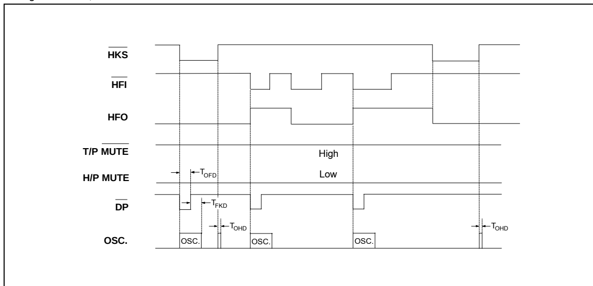
Figure 4(a). Handfree Timing Diagram (with Lock Function)
