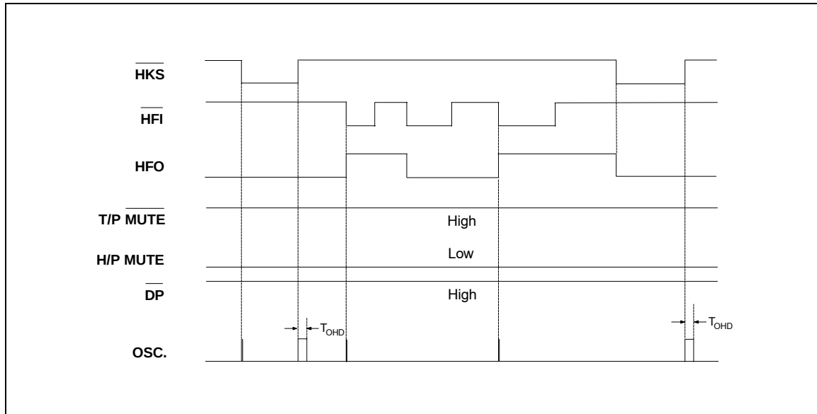
Figure 4(b). Handfree Timing Diagram (without Lock Function)
