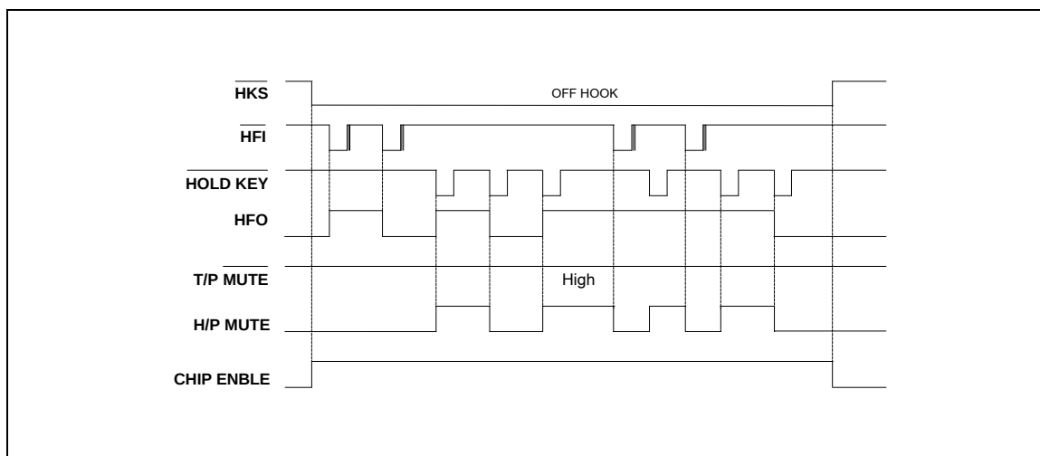
Figure 8(b). Hold and Handfree Timing Diagram
