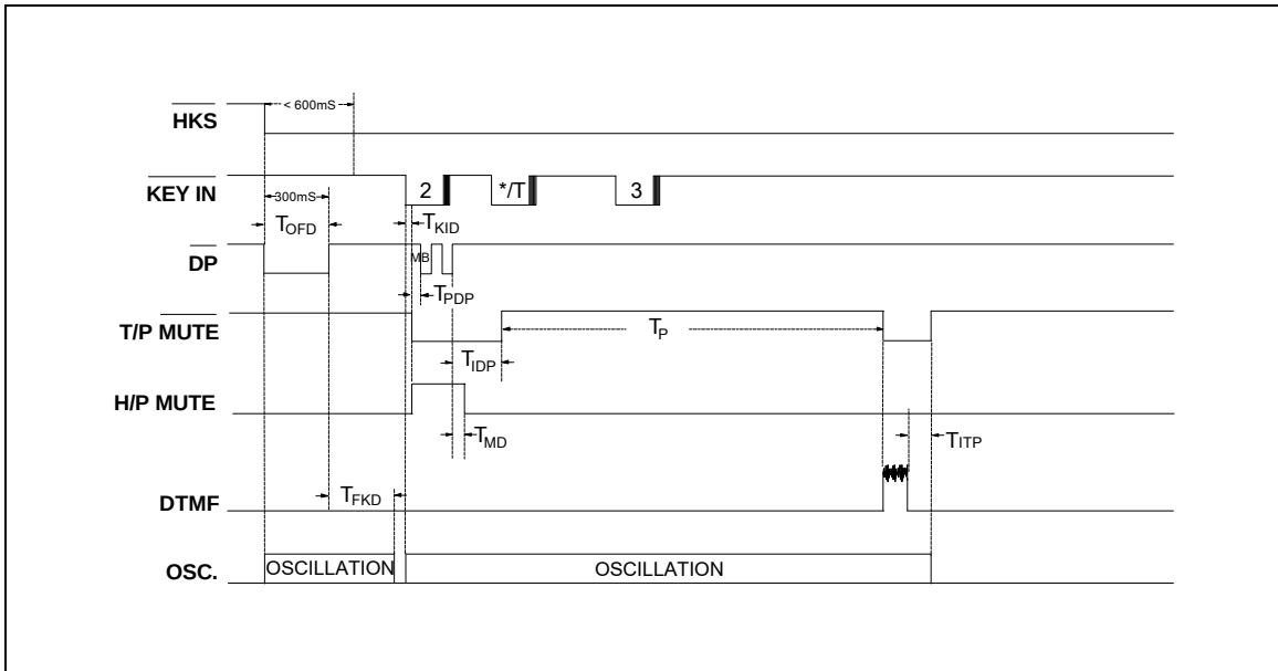
Figure 6(a). Pulse-to-tone Timing Diagram
