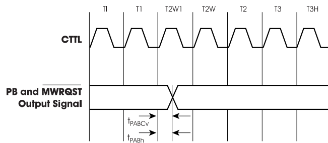
Figure 1-29: Output Signal Timing for Port PB and \overline{\text{MWRQST}}
