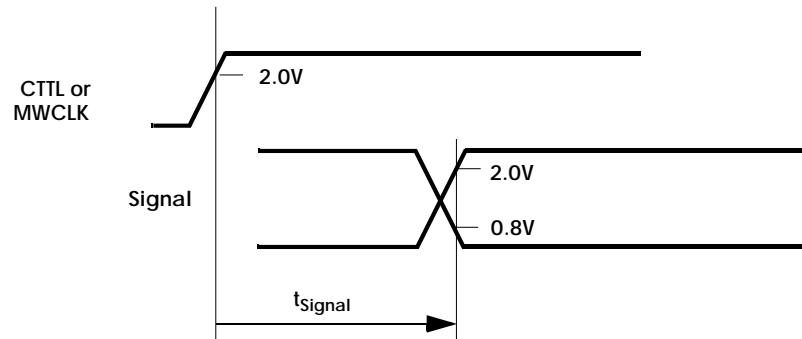
Figure 1-16: Synchronous Output Signals (Valid, Active and Inactive)
