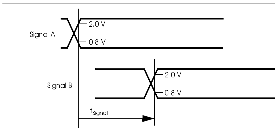
Figure 1-17: Asynchronous Signals
