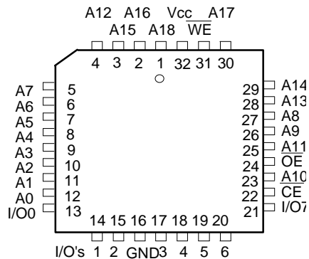
PLCC Top View
