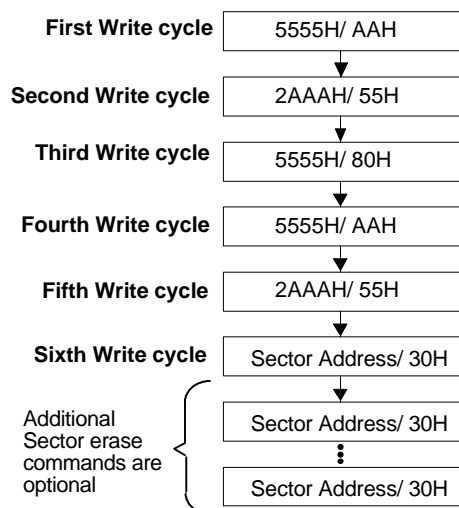
Figure 4. Automated Erase Flow Chart and Sequence
