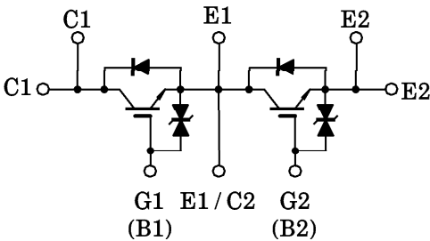
EQUIVALENT CIRCUIT
