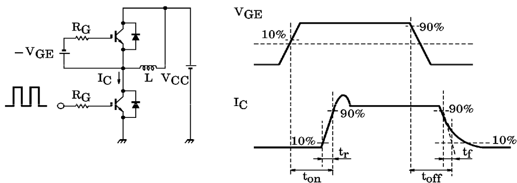
(Note 1) Switching Time Test Circuit & Timing Chart
