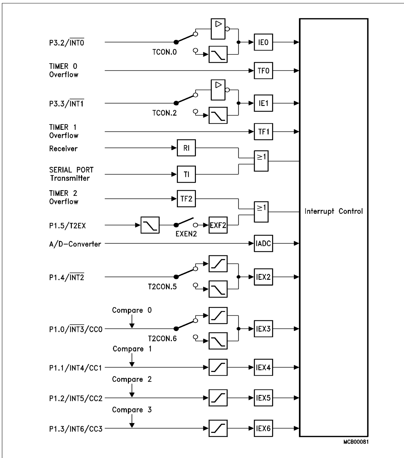
Figure 5 Interrupt Request Sources
