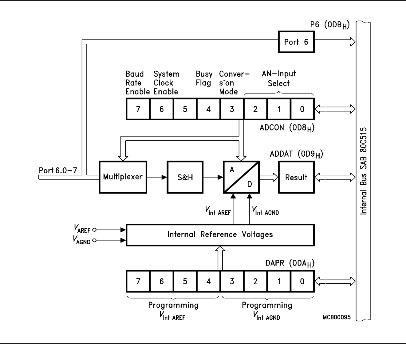
Figure 4 Block Diagram of the A/D Converter
