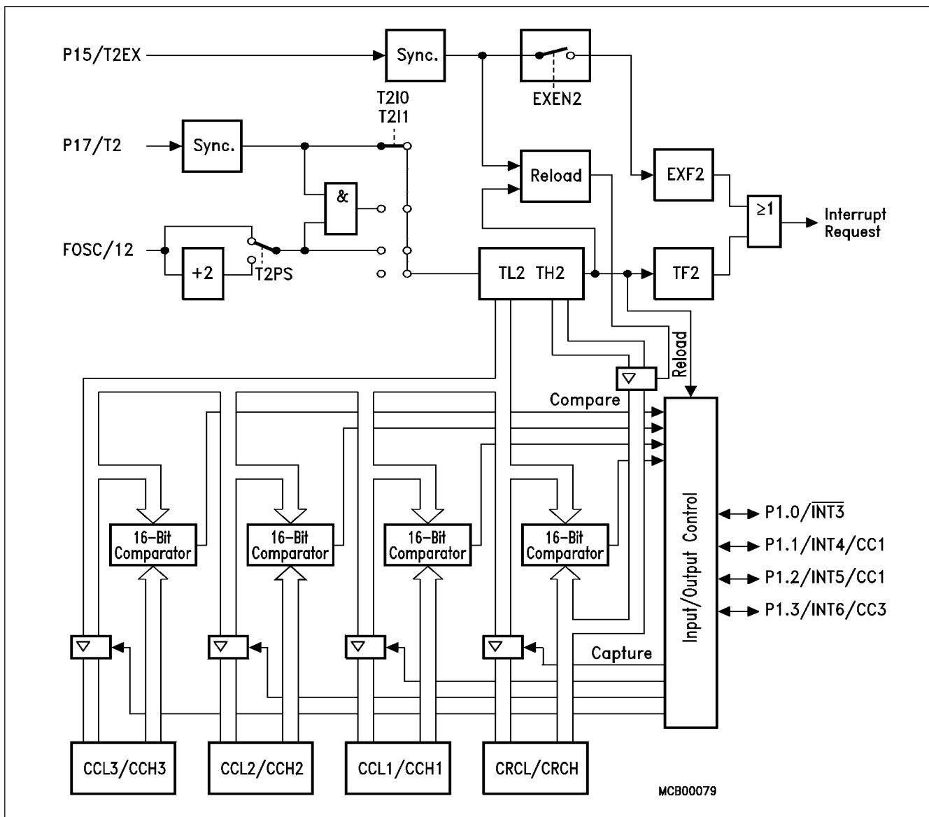
Figure 3 Block Diagram of Timer/Counter 2
