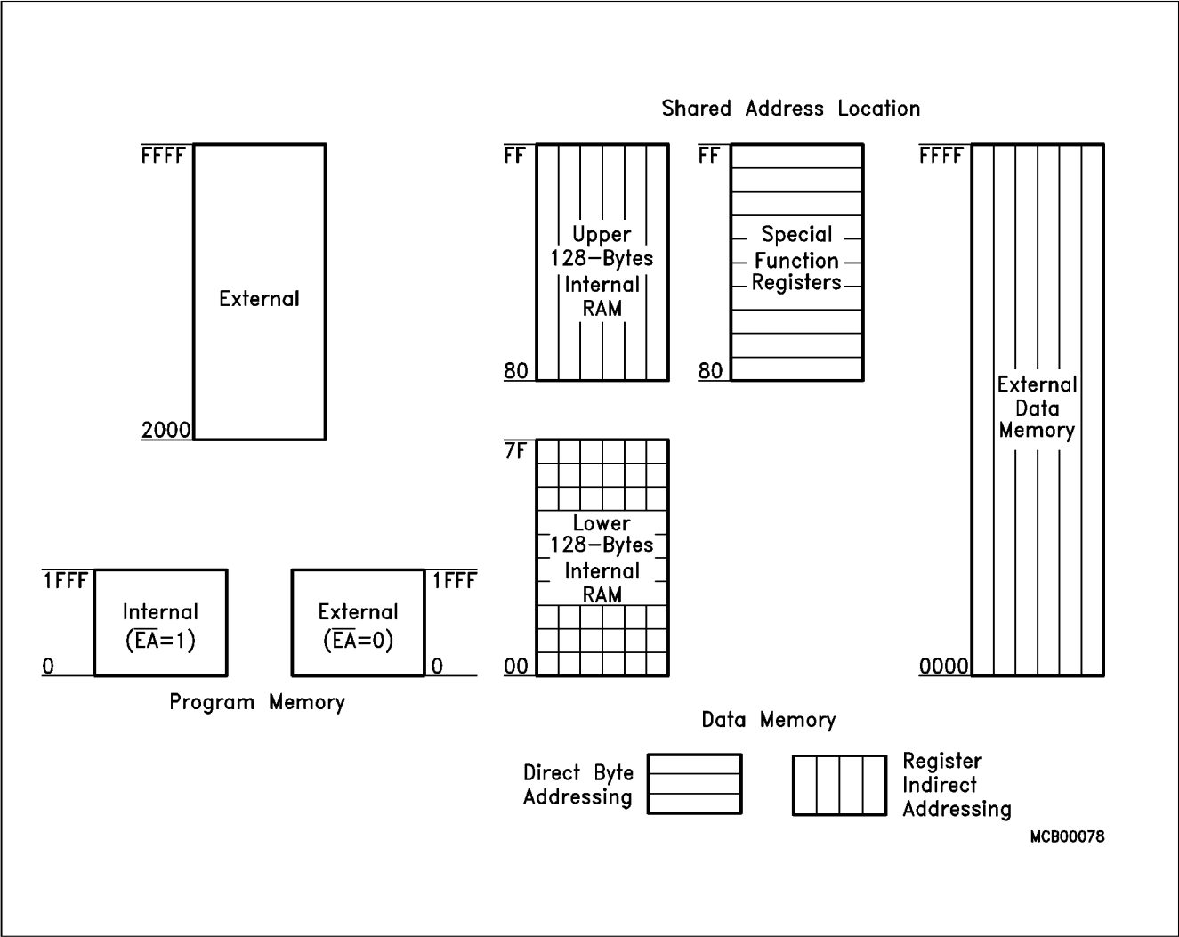
Figure 2 Memory Address Spaces
