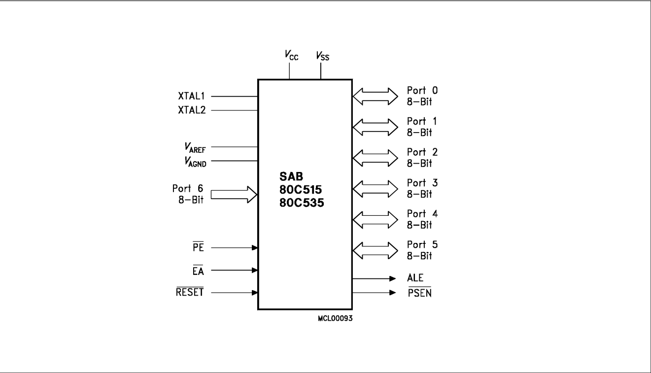
Logic Symbol
