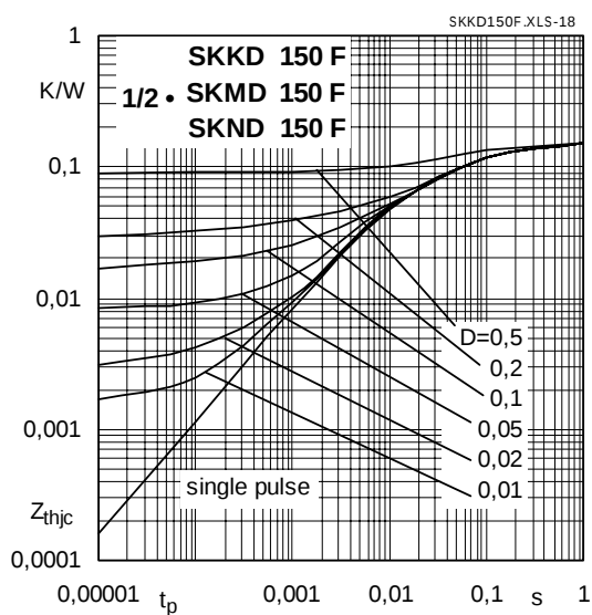
Fig. 18 Typ. transient thermal impedance vs. time
