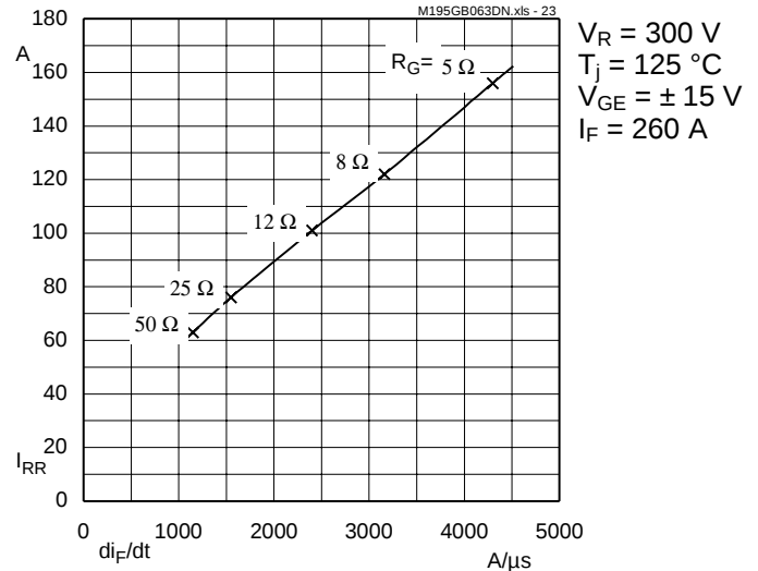
Fig. 23 Typ. CAL diode peak reverse recovery current
