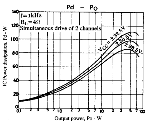
Figure 2. STK4182II Pd - Po ( R_l = 4\Omega )
