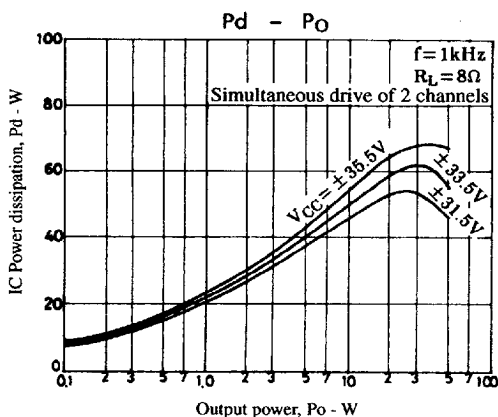
Figure 1. STK4182II Pd - Po ( R_L = 8\Omega )
