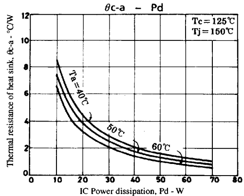
Figure 3. STK4182II θc-a - Pd
