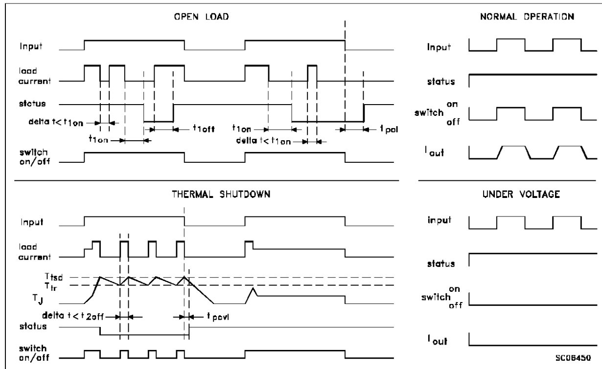
Figure 1: Waveforms
