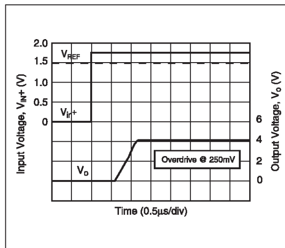
Figure 4 : Transition speed @ 250mV overdrive
