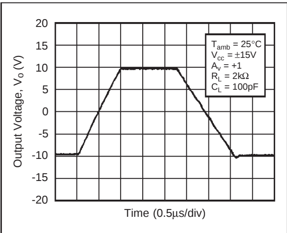
SLEW RATE @ 30V
