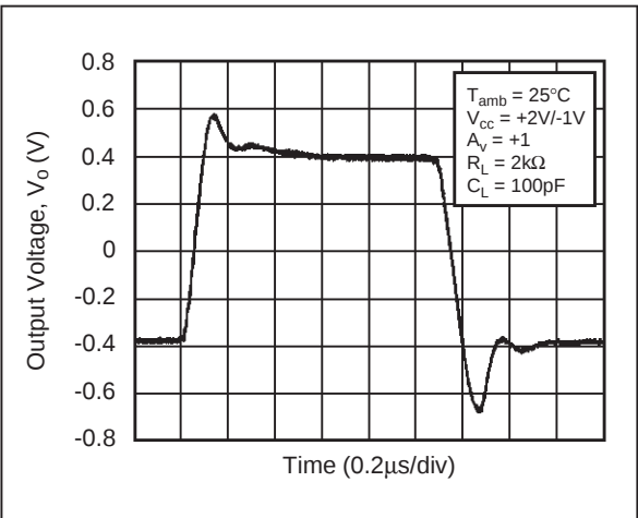
SLEW RATE @ 3V
