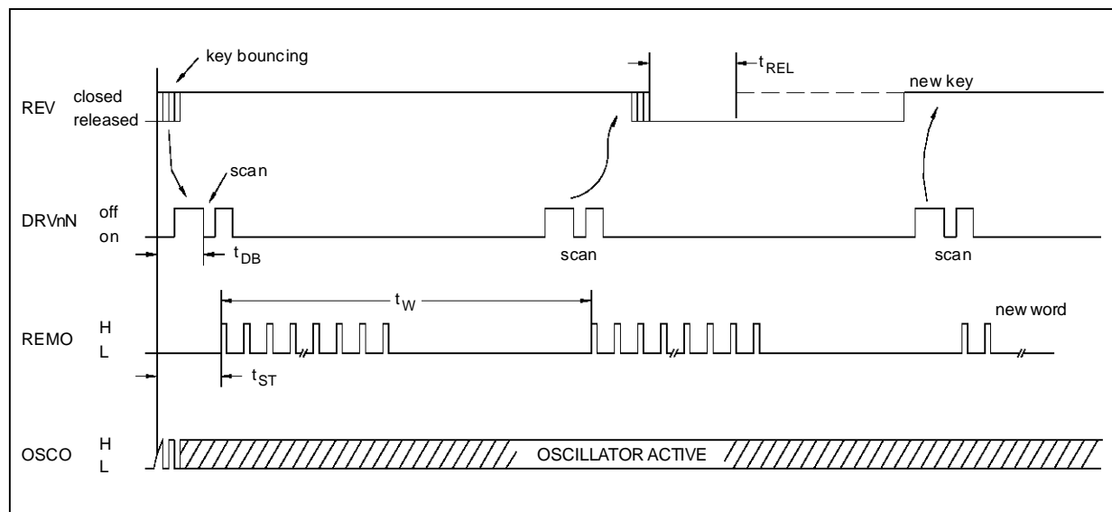
Figure 3 : Single Key-stroke Sequence. Debounce time : t_{DB} = 4 \text{ to } 9 \times t_0 , Start time : t_{ST} = 5 \text{ to } 10 \times t_0 , Minimum release time : t_{REL} = t_0 .
