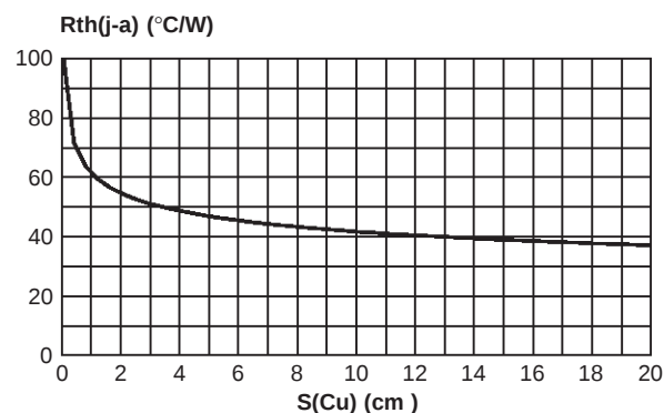
Fig. 8: Thermal resistance junction to ambient versus copper surface under tab (Epoxy printed circuit board FR4, copper thickness: 35 \mu\text{m} ).
