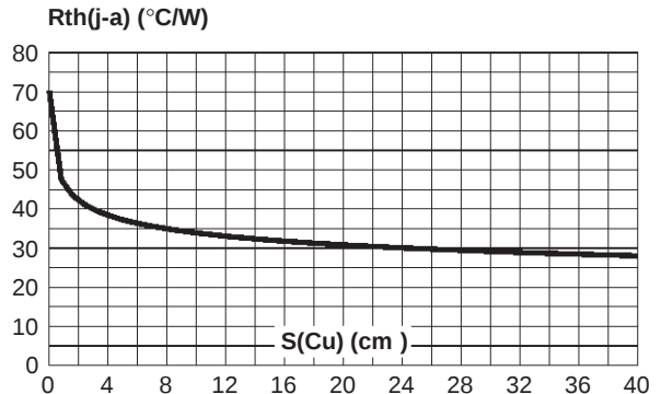
Fig.8 : Thermal resistance junction to ambient versus copper surface under tab (Epoxy printed circuit board FR4, copper thickness : 35\text{ }\mu\text{m} ). (STPS20L25G only)
