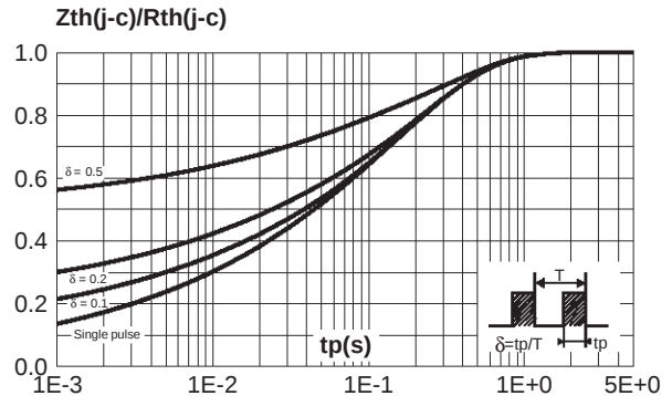
Fig. 4: Relative variation of thermal transient impedance junction to case versus pulse duration (per diode).
