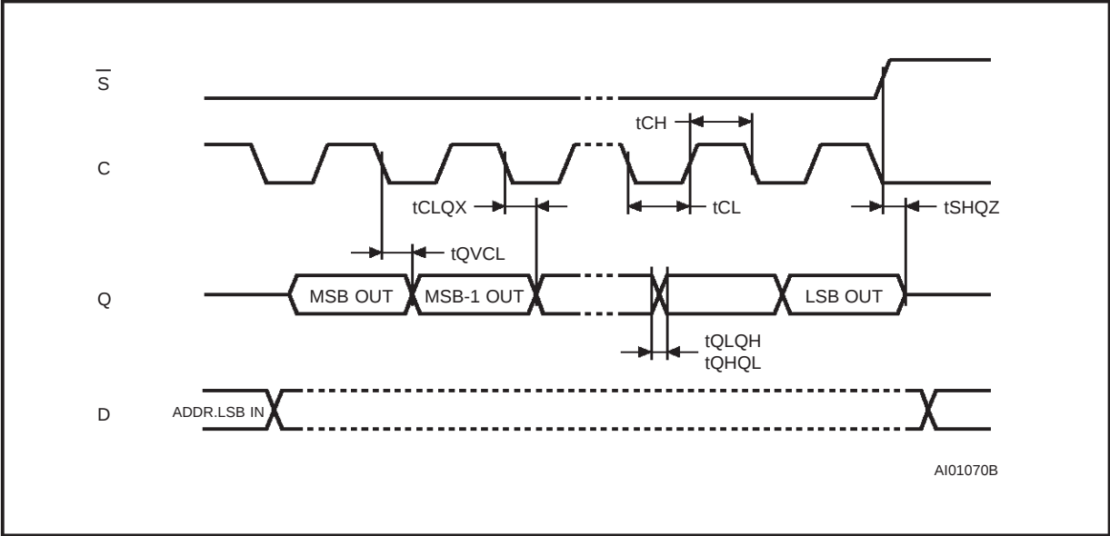
Figure 5. Output Timing
