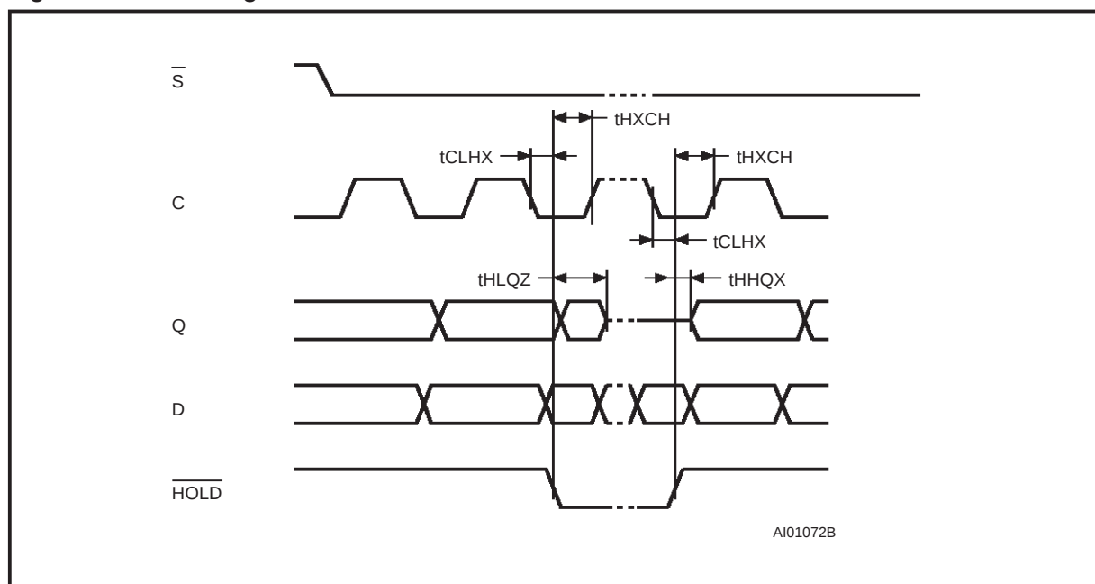
Figure 7. Hold Timing
