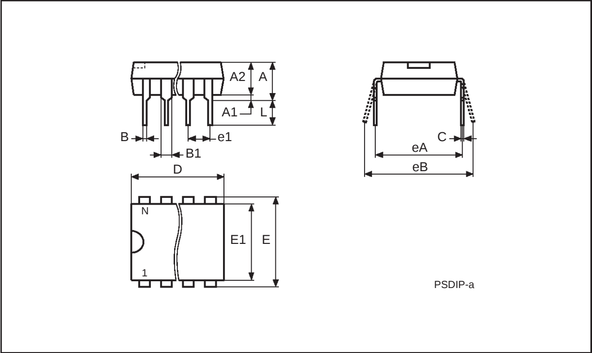
PSDIP8
