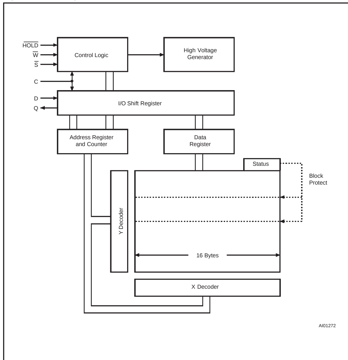
Figure 3. Block Diagram
