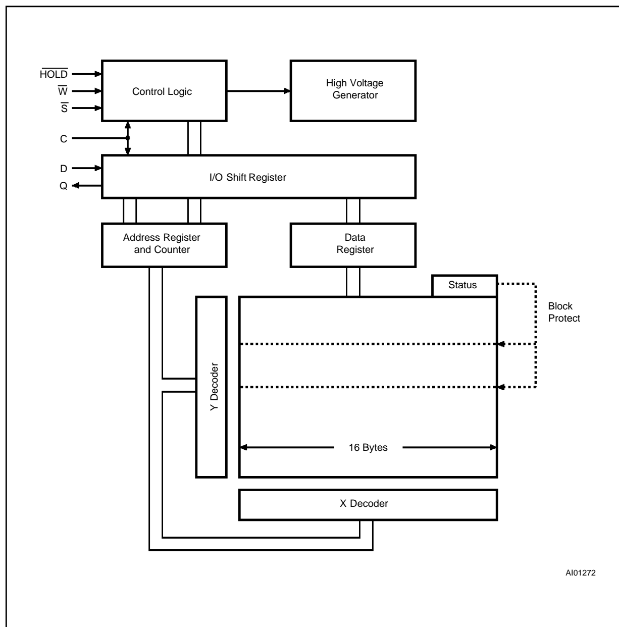
Figure 3. Block Diagram
