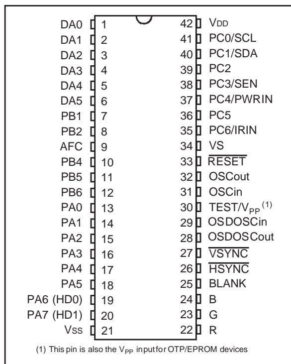
Figure 3. ST63E87, T87 Pin configuration
