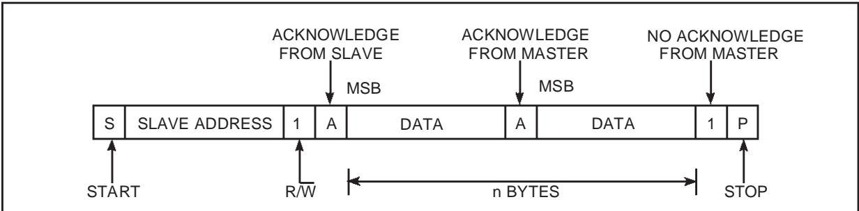
Figure 23. I C Master Reads Slave Immediately After First Byte (Read Mode)
