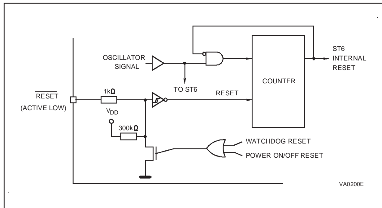
Figure 16. Reset Circuit
