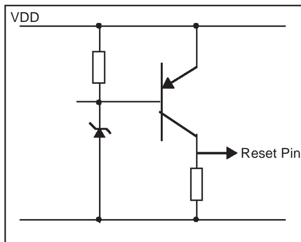
Figure 4. Reset Network
