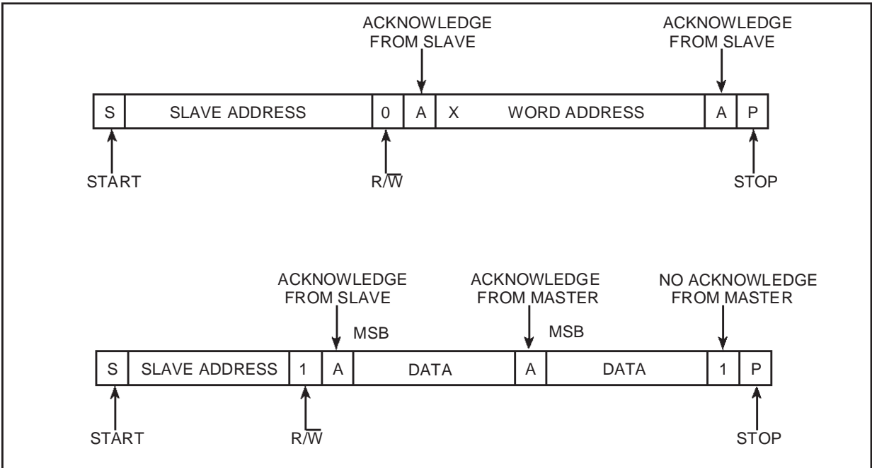
Figure 24. I C Master Reads After Setting Slave Register Address (Write Address, Read Data)
