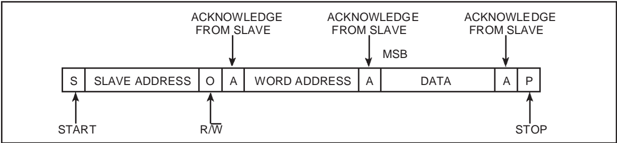
Figure 22. I C Master Transmit to Slave Receiver (Write Mode)
