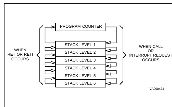
Figure 5. Stack Operation
