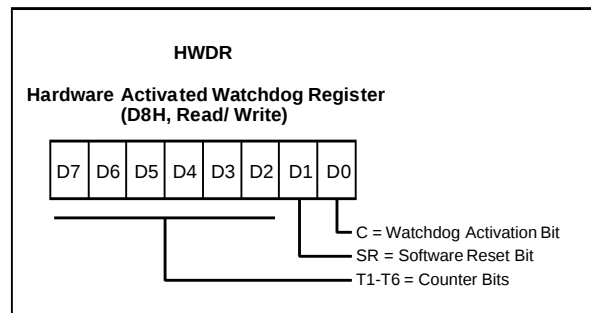
Figure 37. Watchdog Register
