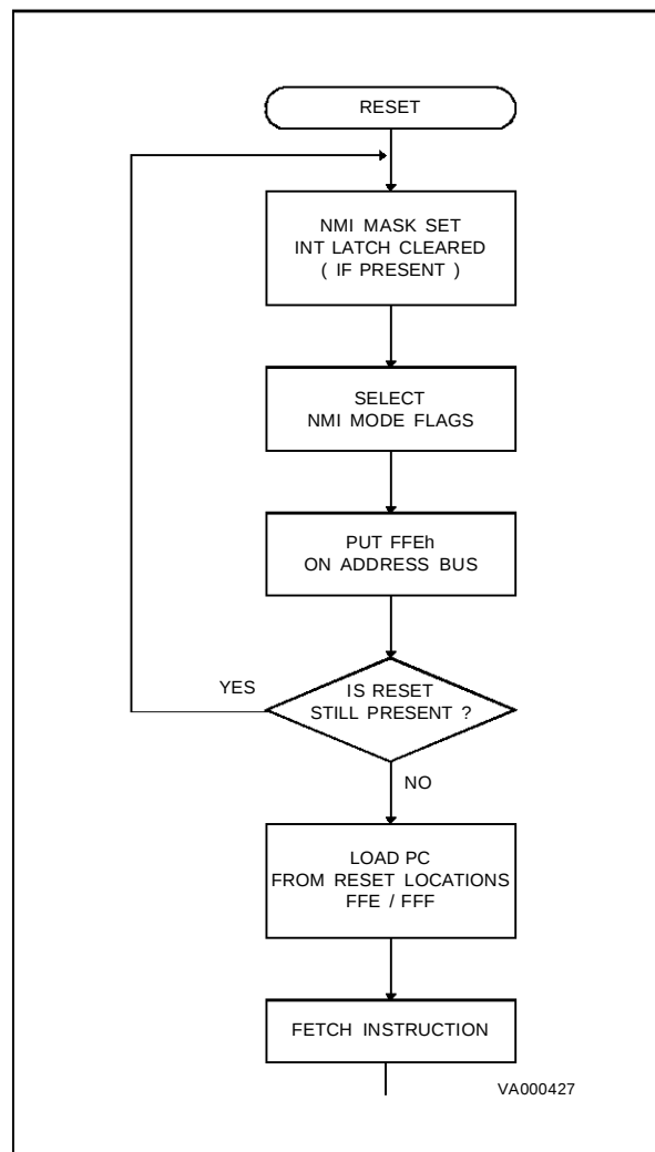
Figure 21. Reset &amp; Interrupt Processing Flow-Chart
