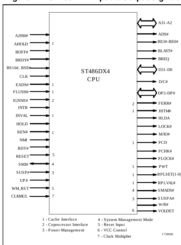
Figure 1-1. ST486 DX4 Input & Output Signals.
