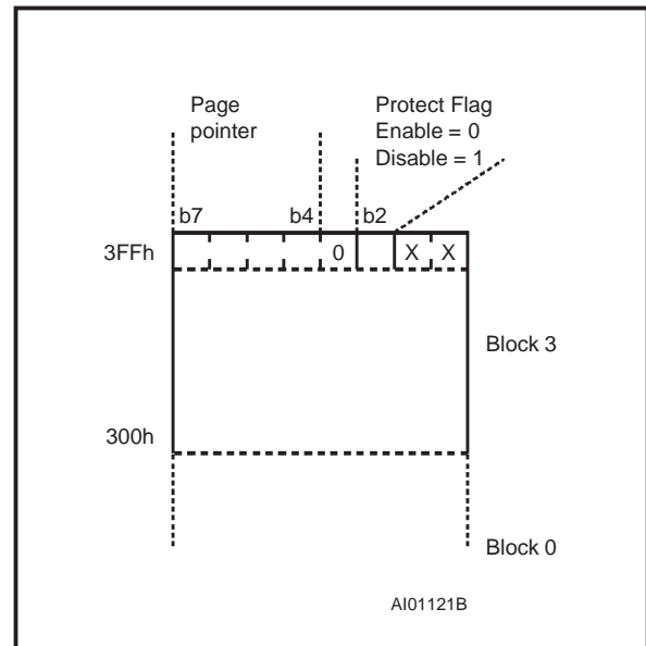
Figure 7. Memory Protection
