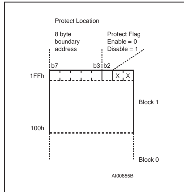
Figure 7. Memory Protection
