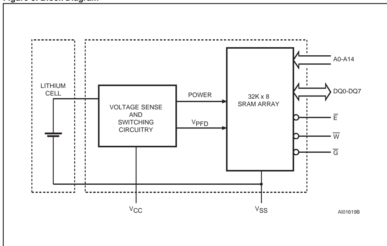
Figure 3. Block Diagram
