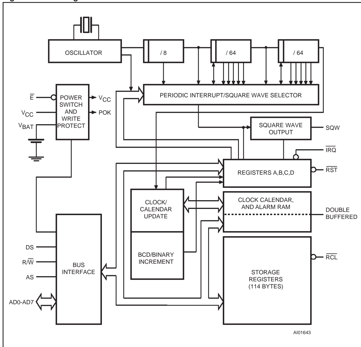
Figure 4. Block Diagram
