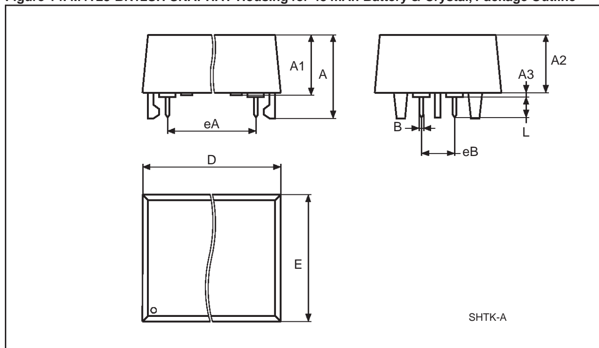
Figure 14. M4T28-BR12SH SNAPHAT Housing for 48 mAh Battery &amp; Crystal, Package Outline
