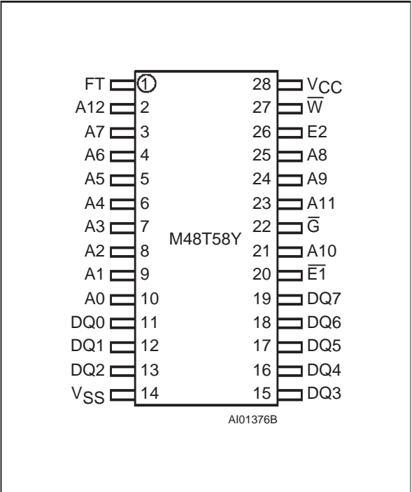
Figure 2B. SOIC Connections
