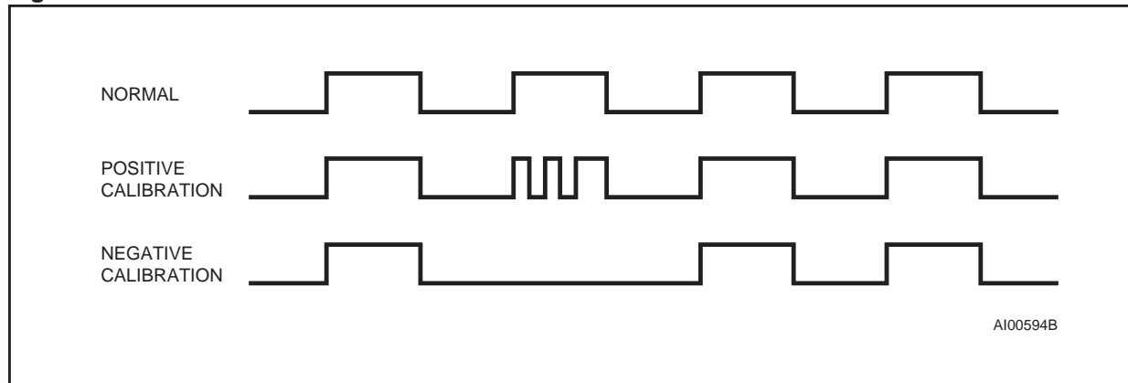
Figure 9. Clock Calibration
