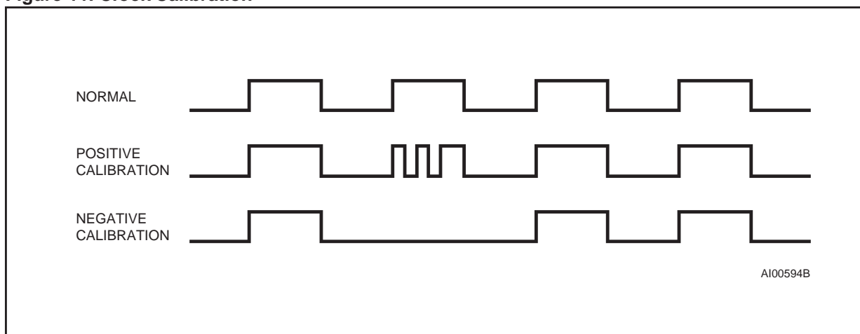
Figure 11. Clock Calibration
