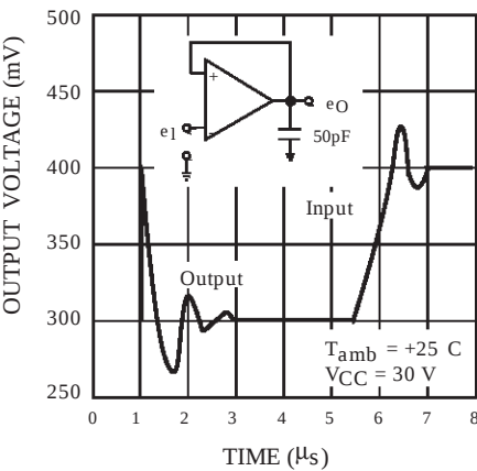
VOLTAGE FOLLOWER PULSSE RESPONSE (SMALL SIGNAL)
