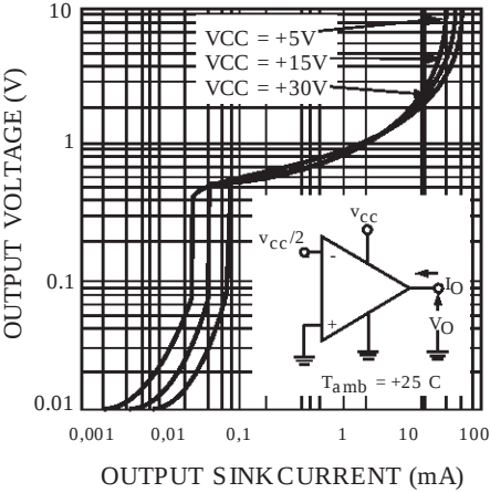
OUTPUT CHARACTERISTICS
