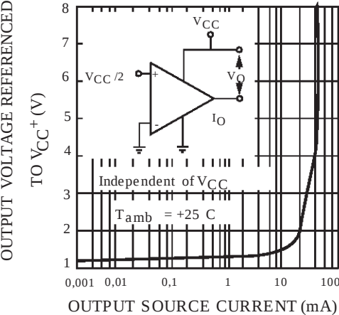
OUTPUT CHARACTERISTICS
