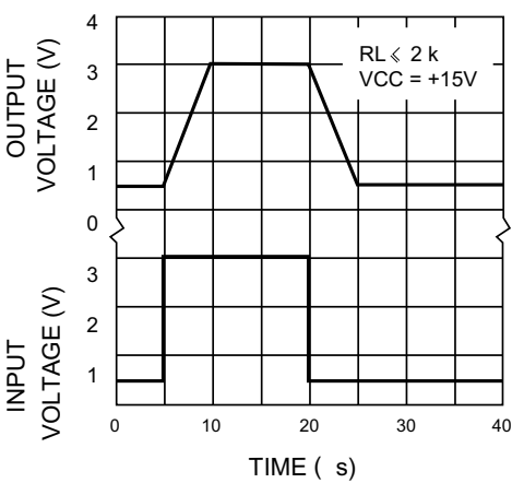
VOLTA FOLLOWER PULSE RESPONSE
