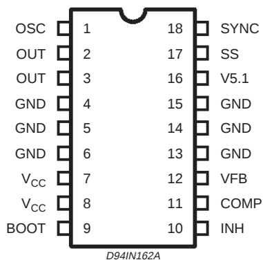
POWERDIP (12+3+3)
