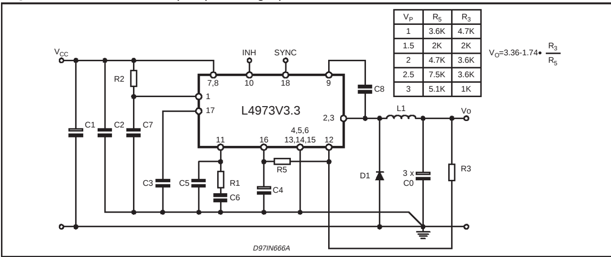
Figure 32: 3.5A at VO < 3.3V (see part list fig. 1)
