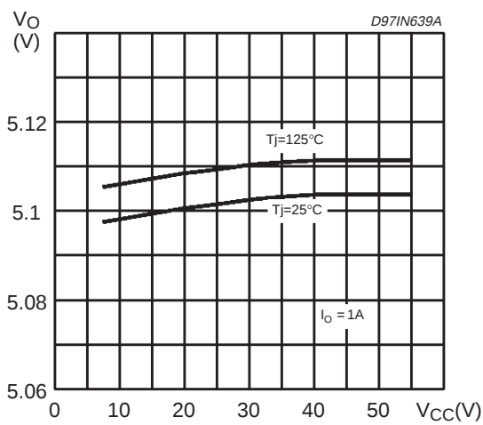
Figure 9: Line Regulation (see fig. 1)
