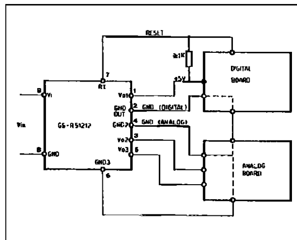
Figure 3. Typical application
