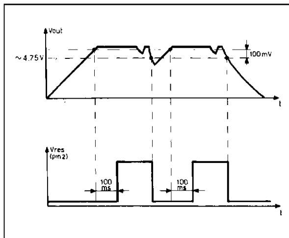
Figure 2. Reset Operation
