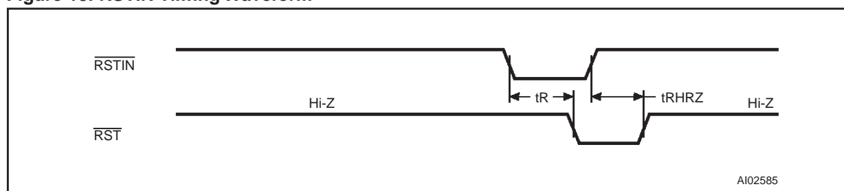
Figure 13. \overline{\text{RSTIN}} Timing Waveform
