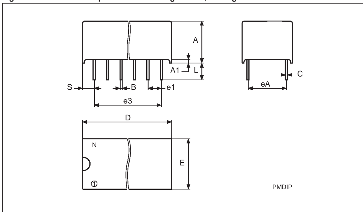
Figure 19. PMLDIP36 - 36 pin Plastic DIP Long Module, Package Outline
