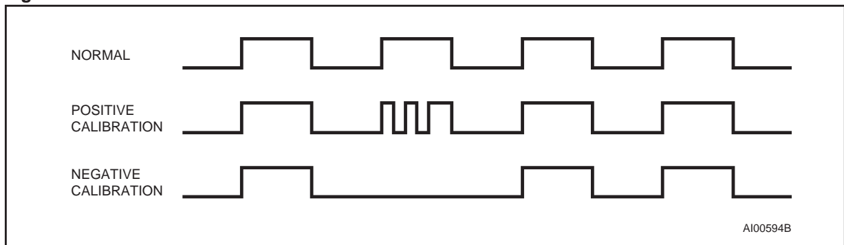
Figure 15. Calibration Waveform
