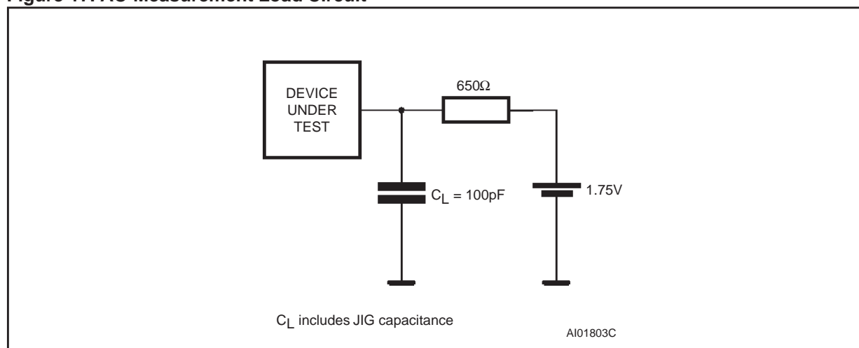
Figure 17. AC Measurement Load Circuit
