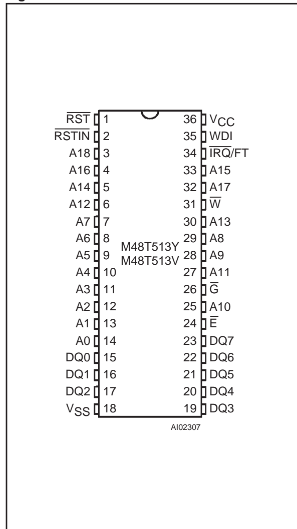
Figure 4. DIP Connections
