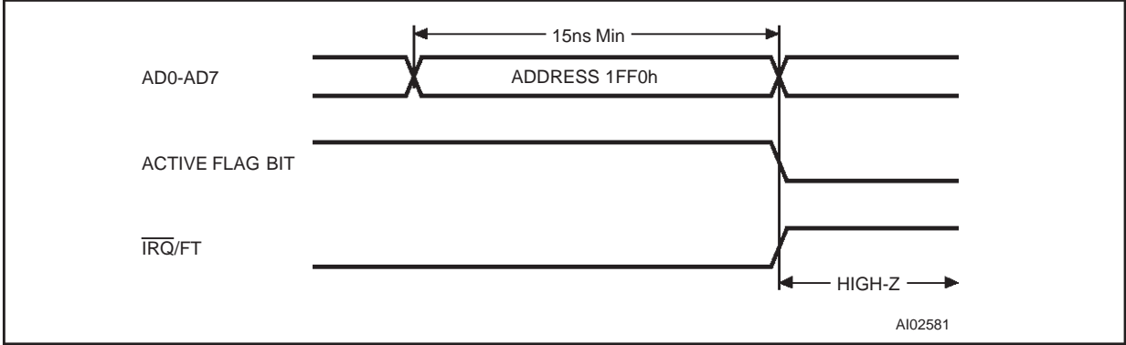
Figure 11. Alarm Interrupt Reset Waveform
