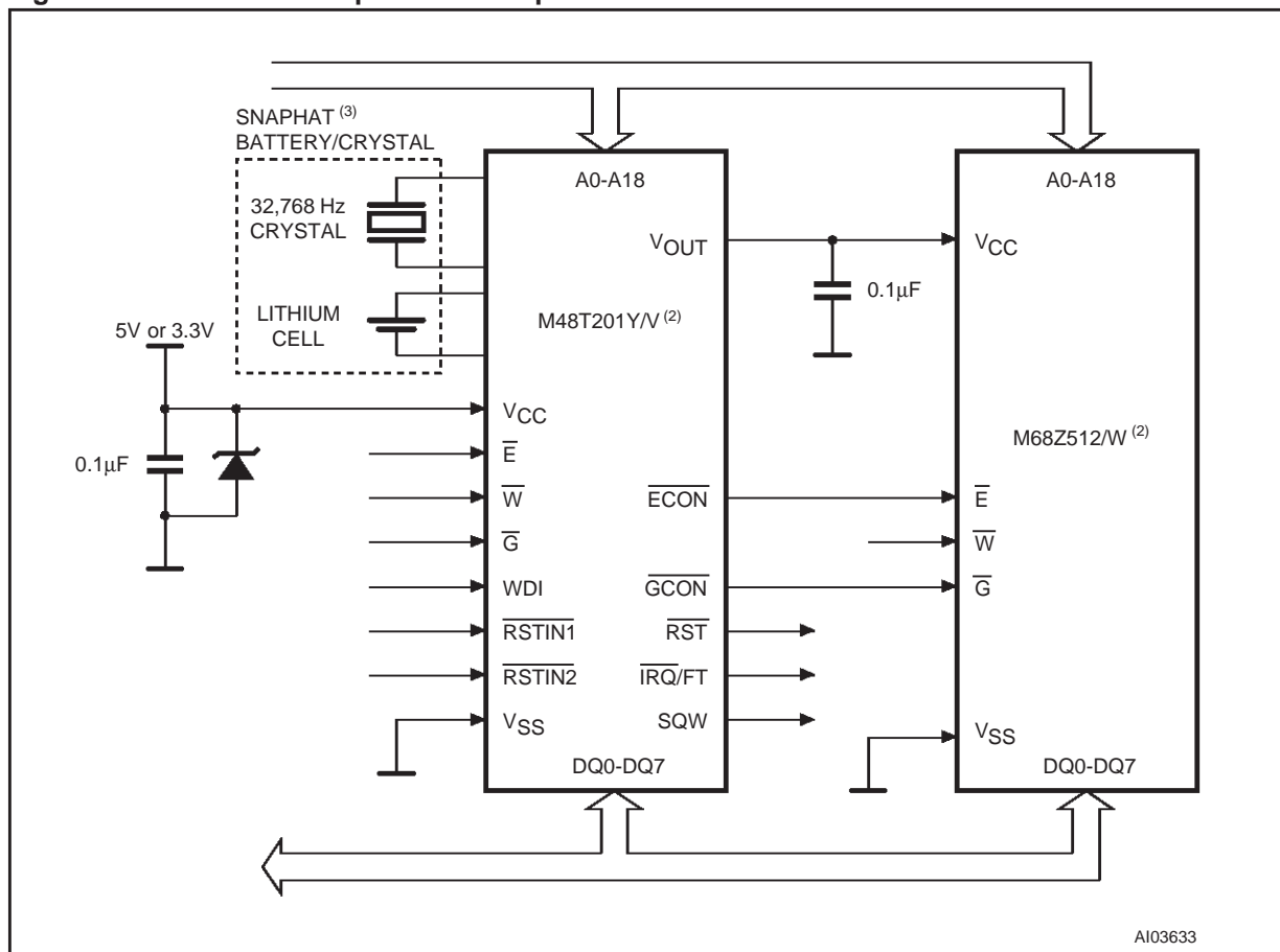
Figure 6. Hardware Hookup for SMT Chipset
