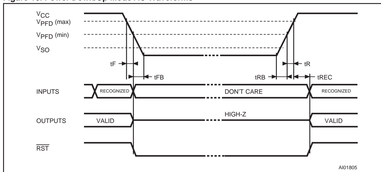
Figure 18. Power Down/Up Mode AC Waveforms
