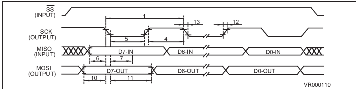
Figure 74. SPI Master Timing Diagram CPHA=0, CPOL=1
