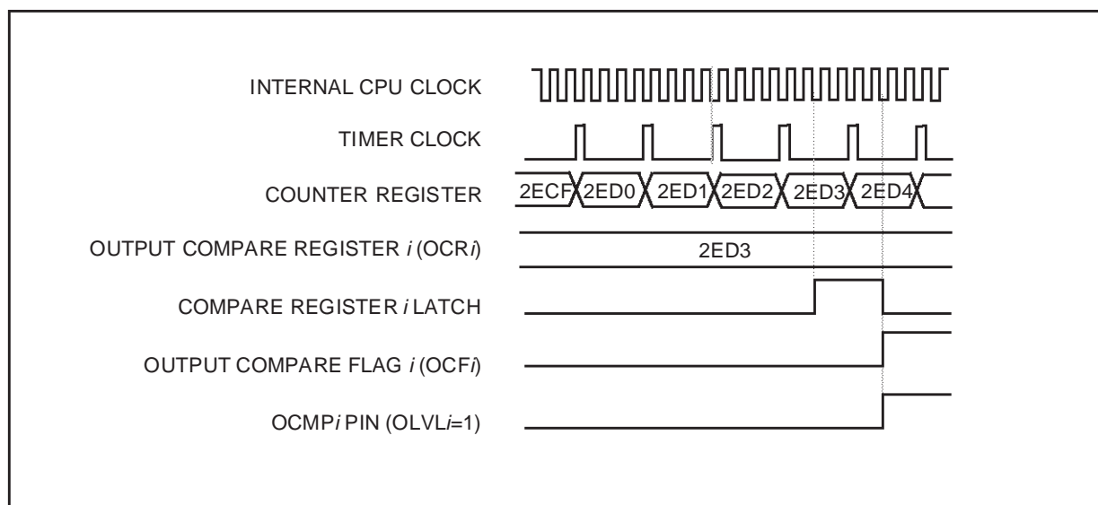
Figure 41. Output Compare Timing Diagram, f_{\text{TIMER}} = f_{\text{CPU}}/4
