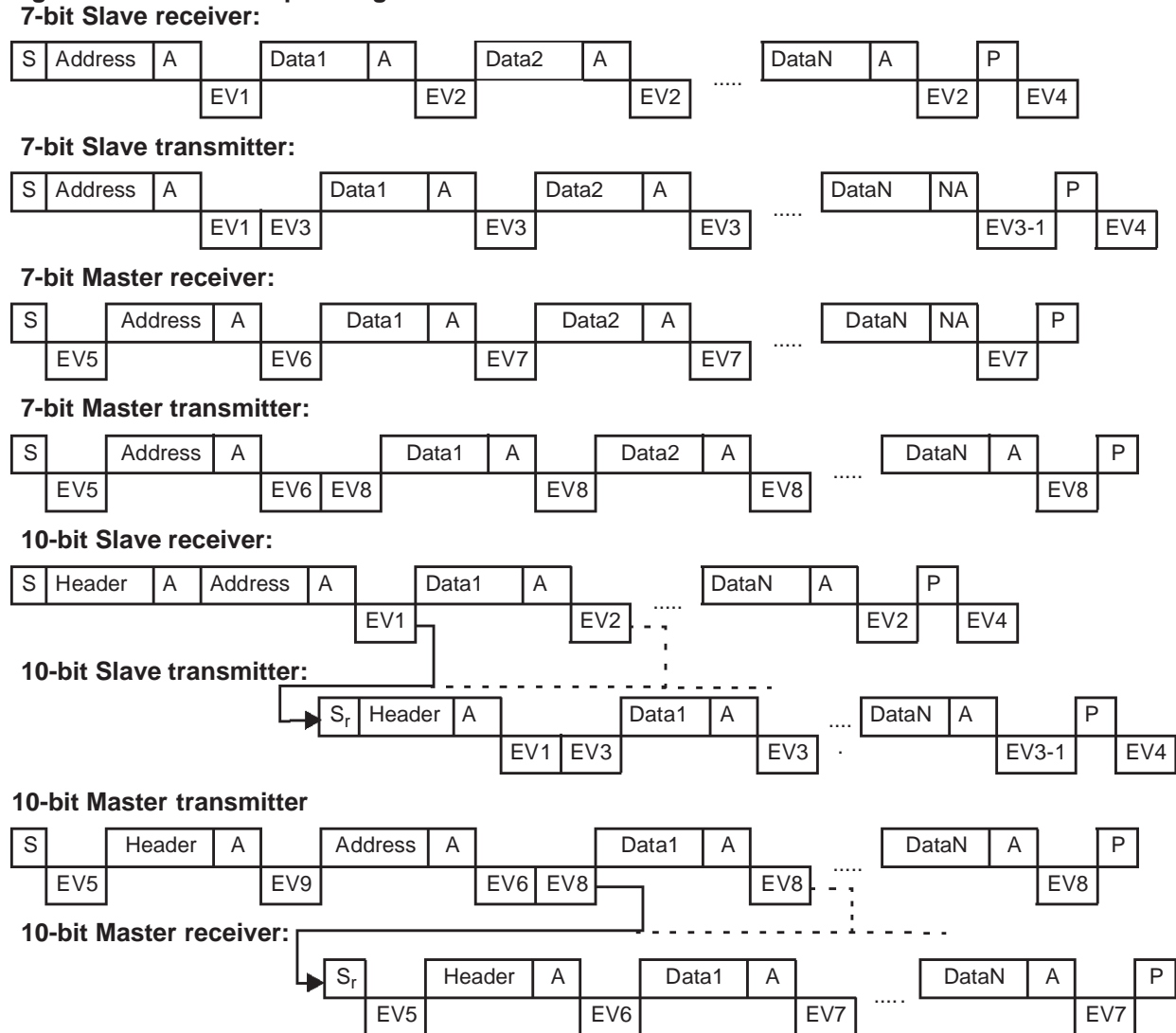
Figure 62. Transfer Sequencing
