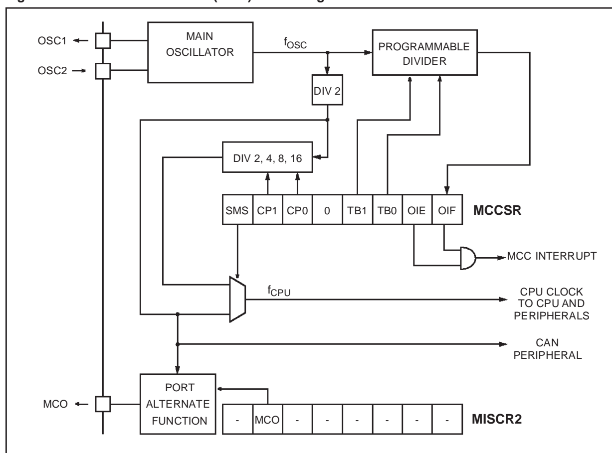
Figure 14. Main Clock Controller (MCC) Block Diagram
