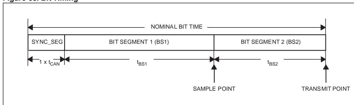
Figure 68. Bit Timing
