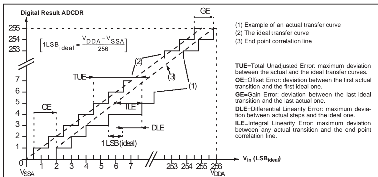
ADC Analog to Digital Converter (8-bit) for ST72E/T589BW5 and ST72E/T589CW5 devices
