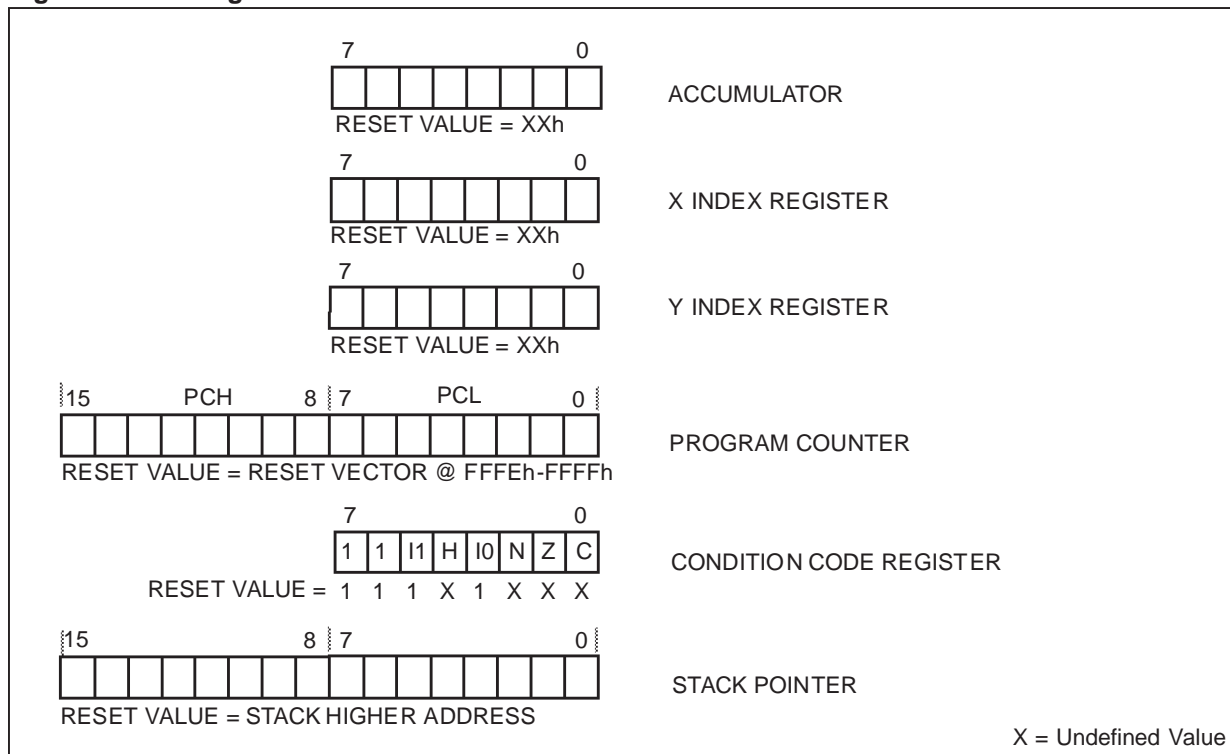
Figure 4. CPU Registers
