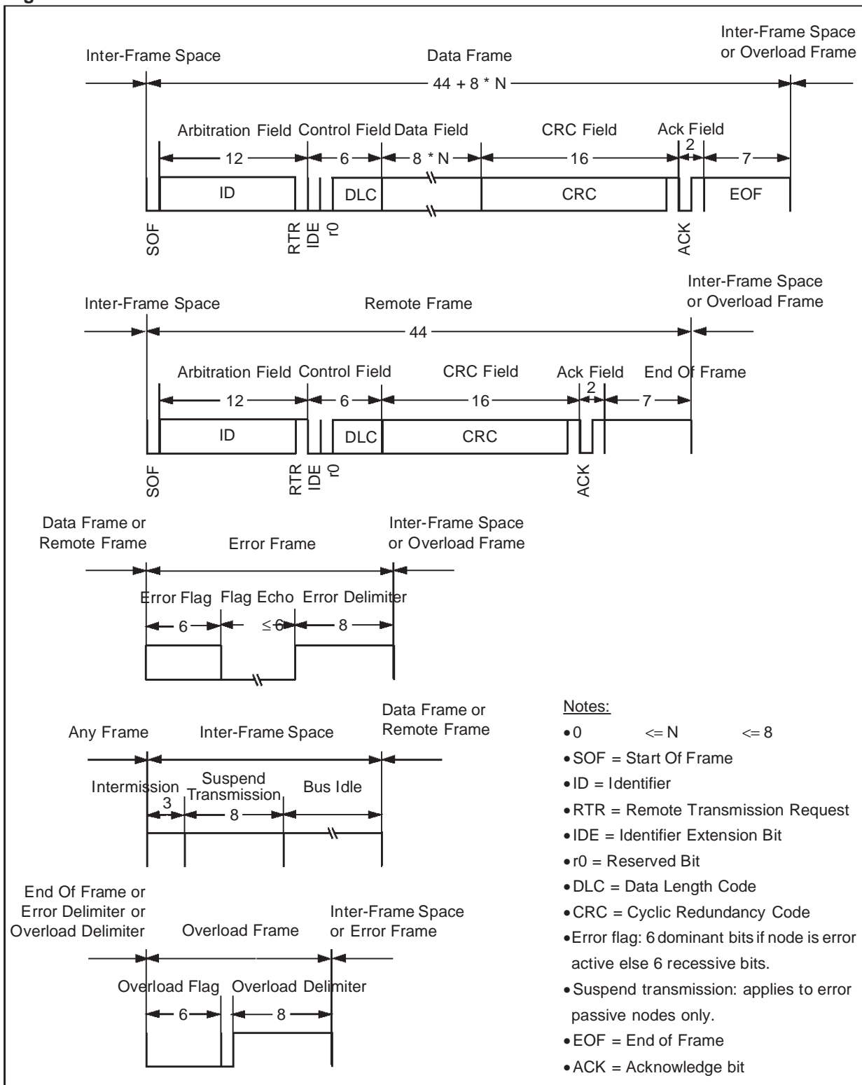
Figure 65. CAN Frames
