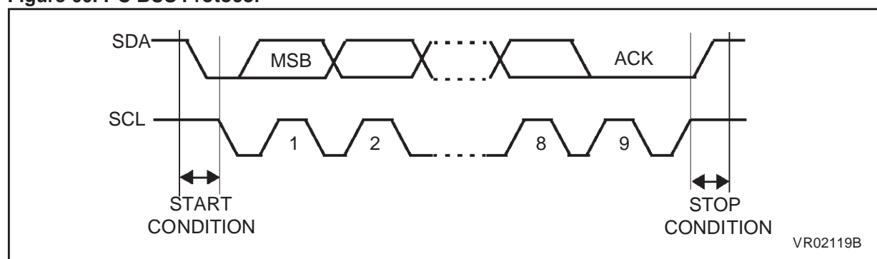
Figure 60. I 2 C BUS Protocol
