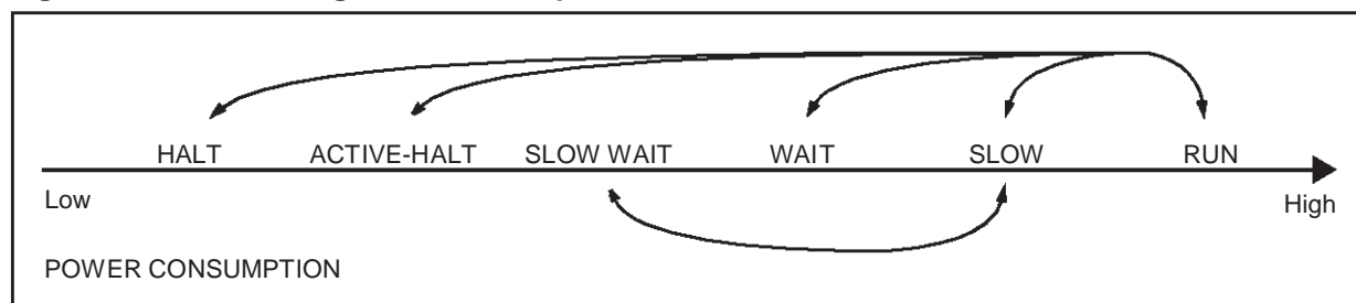
Figure 20. Power saving mode consumption / transitions
