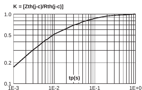
Fig. 3-1: Relative variation of thermal impedance junction to case versus pulse duration.
