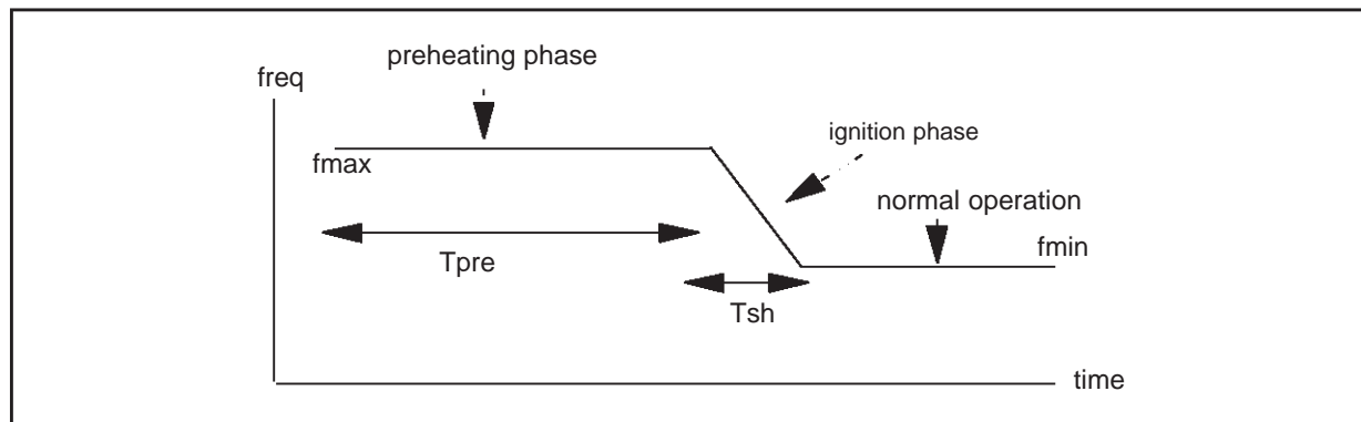
Figure 2. Frequency shift
