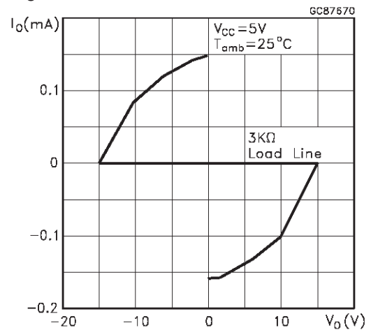
Figure 4 : Driver Output Current vs Output Voltage
