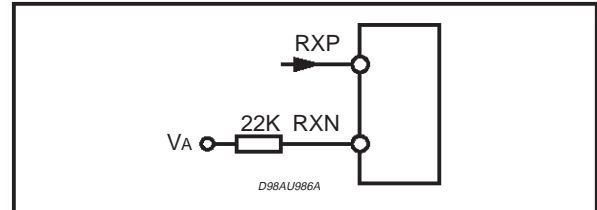
Figure 23. Consumer Input Circuit
