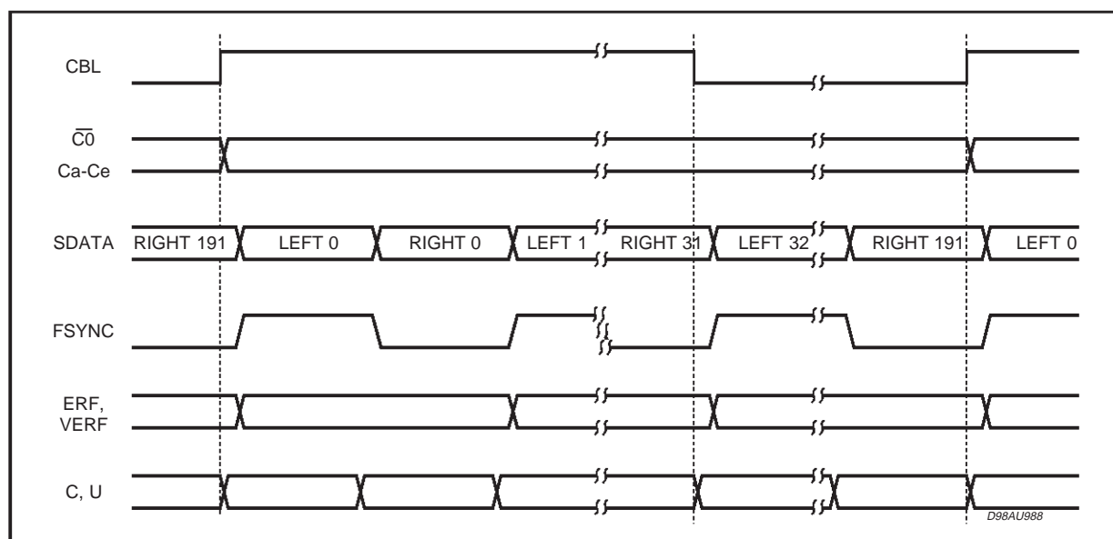
Figure 19. CBL Timing
