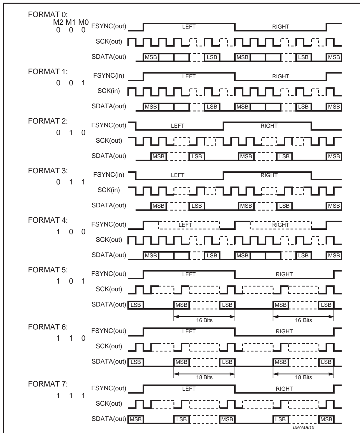
Figure 3. Audio Serial Port Formats.
